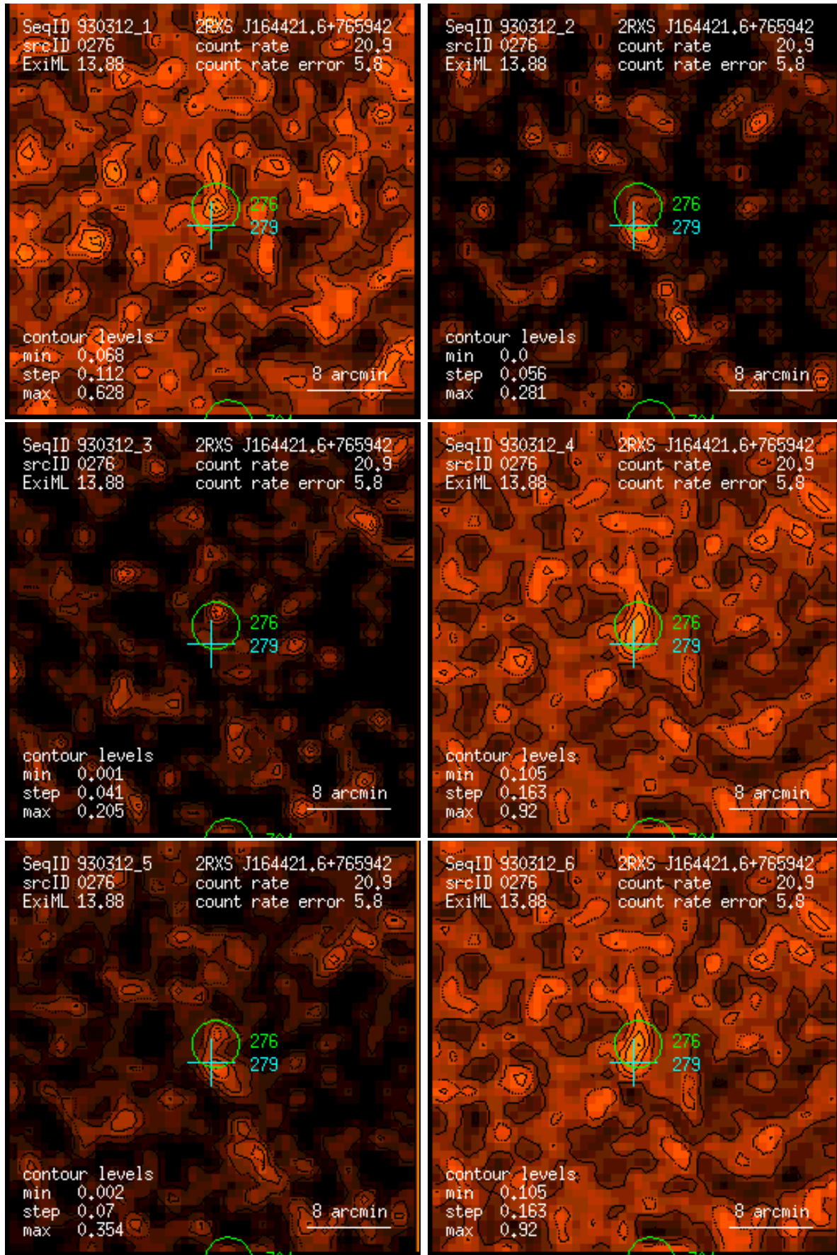
Figure 276: RASS 930312: detection 0276: band rate images, Gaussian filter: (1) PSPC channels 11 – 41, (2) 52 – 90, (3) 91 – 201, (4) 11 – 235, (5) 52 – 201, (6) 11 – 201. Broad band rates in counts/ks. Band rate contour levels in counts/ks/arcmin 2 .
