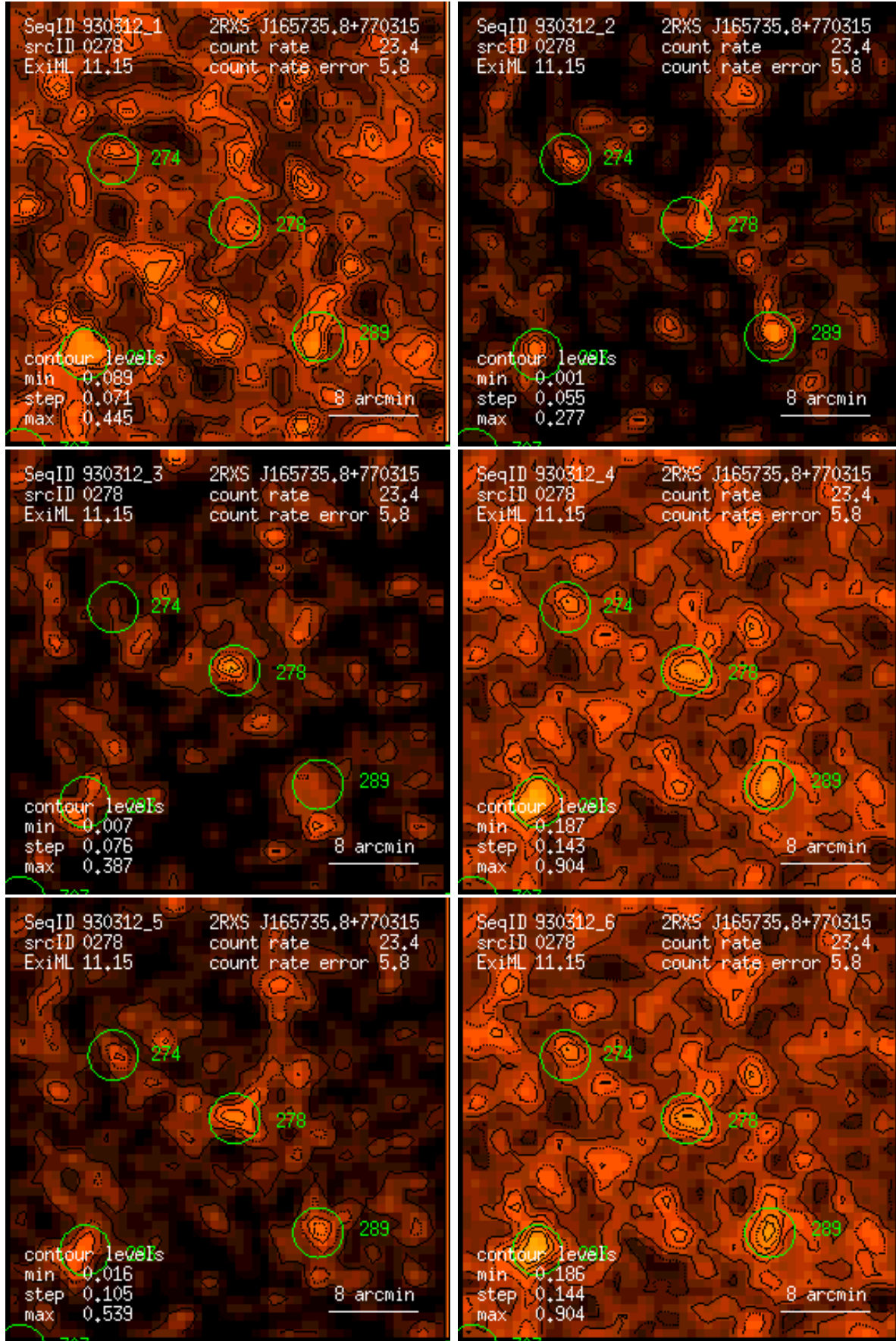
Figure 278: RASS 930312: detection 0278: band rate images, Gaussian filter: (1) PSPC channels 11 – 41, (2) 52 – 90, (3) 91 – 201, (4) 11 – 235, (5) 52 – 201, (6) 11 – 201. Broad band rates in counts/ks. Band rate contour levels in counts/ks/arcmin 2 .
