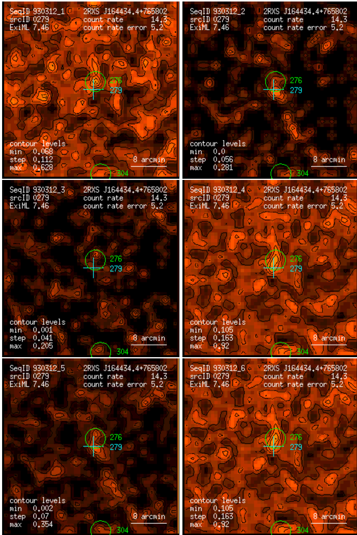
Figure 279: RASS 930312: detection 0279: band rate images, Gaussian filter: (1) PSPC channels 11 – 41, (2) 52 – 90, (3) 91 – 201, (4) 11 – 235, (5) 52 – 201, (6) 11 – 201. Broad band rates in counts/ks. Band rate contour levels in counts/ks/arcmin 2 .
