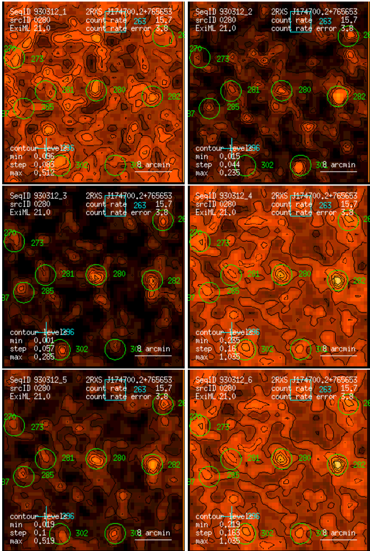
Figure 280: RASS 930312: detection 0280: band rate images, Gaussian filter: (1) PSPC channels 11 – 41, (2) 52 – 90, (3) 91 – 201, (4) 11 – 235, (5) 52 – 201, (6) 11 – 201. Broad band rates in counts/ks. Band rate contour levels in counts/ks/arcmin 2 .
