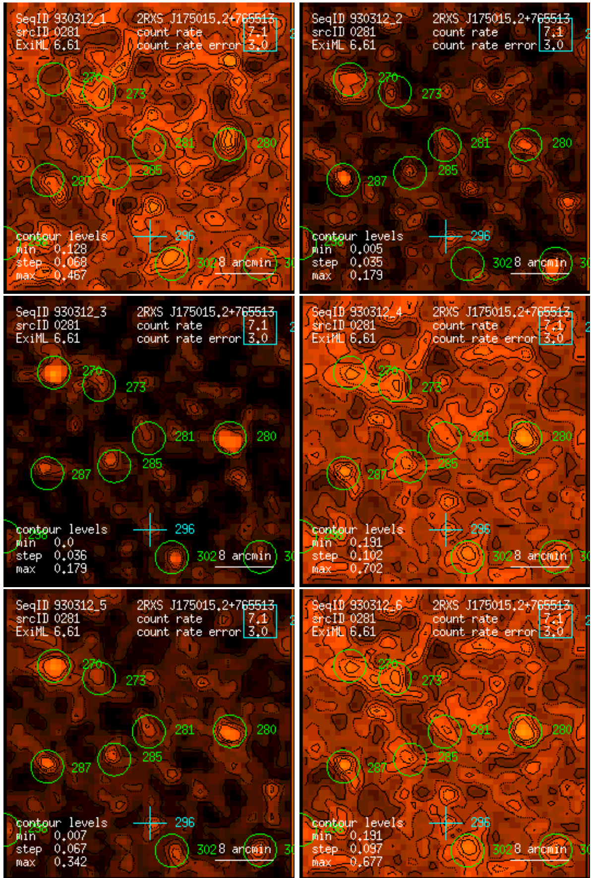
Figure 281: RASS 930312: detection 0281: band rate images, Gaussian filter: (1) PSPC channels 11 – 41, (2) 52 – 90, (3) 91 – 201, (4) 11 – 235, (5) 52 – 201, (6) 11 – 201. Broad band rates in counts/ks. Band rate contour levels in counts/ks/arcmin 2 .
