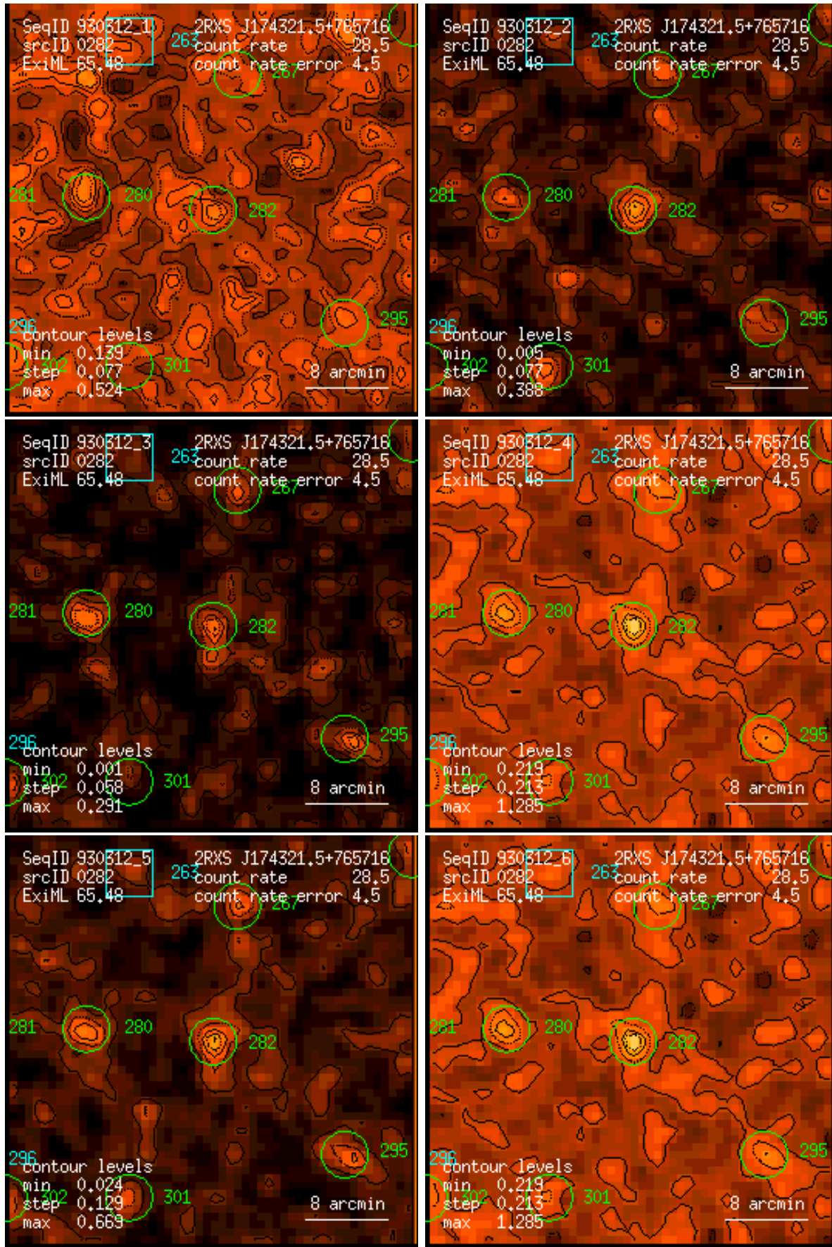
Figure 282: RASS 930312: detection 0282: band rate images, Gaussian filter: (1) PSPC channels 11 – 41, (2) 52 – 90, (3) 91 – 201, (4) 11 – 235, (5) 52 – 201, (6) 11 – 201. Broad band rates in counts/ks. Band rate contour levels in counts/ks/arcmin 2 .
