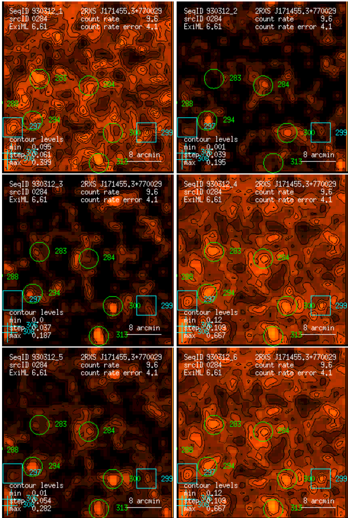
Figure 284: RASS 930312: detection 0284: band rate images, Gaussian filter: (1) PSPC channels 11 – 41, (2) 52 – 90, (3) 91 – 201, (4) 11 – 235, (5) 52 – 201, (6) 11 – 201. Broad band rates in counts/ks. Band rate contour levels in counts/ks/arcmin 2 .
