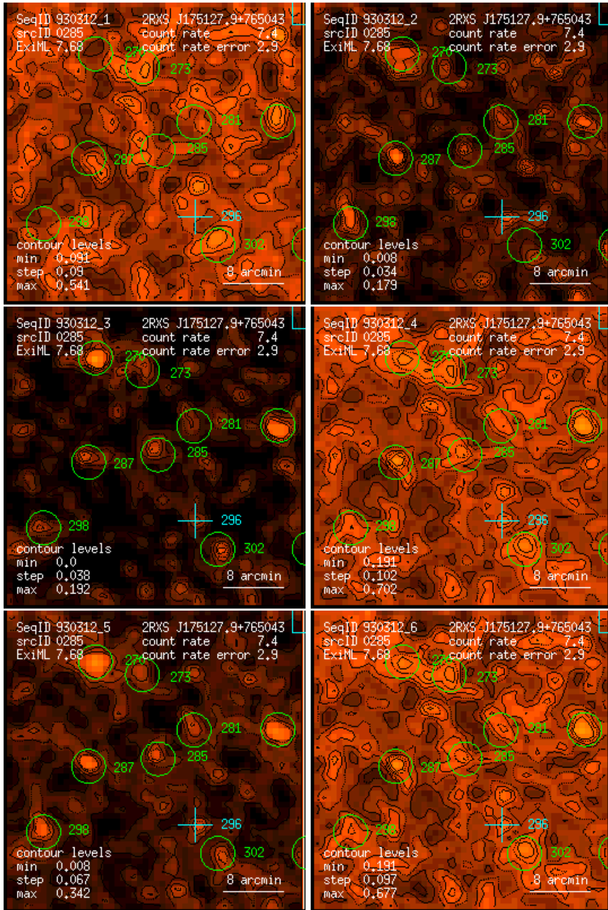
Figure 285: RASS 930312: detection 0285: band rate images, Gaussian filter: (1) PSPC channels 11 – 41, (2) 52 – 90, (3) 91 – 201, (4) 11 – 235, (5) 52 – 201, (6) 11 – 201. Broad band rates in counts/ks. Band rate contour levels in counts/ks/arcmin 2 .
