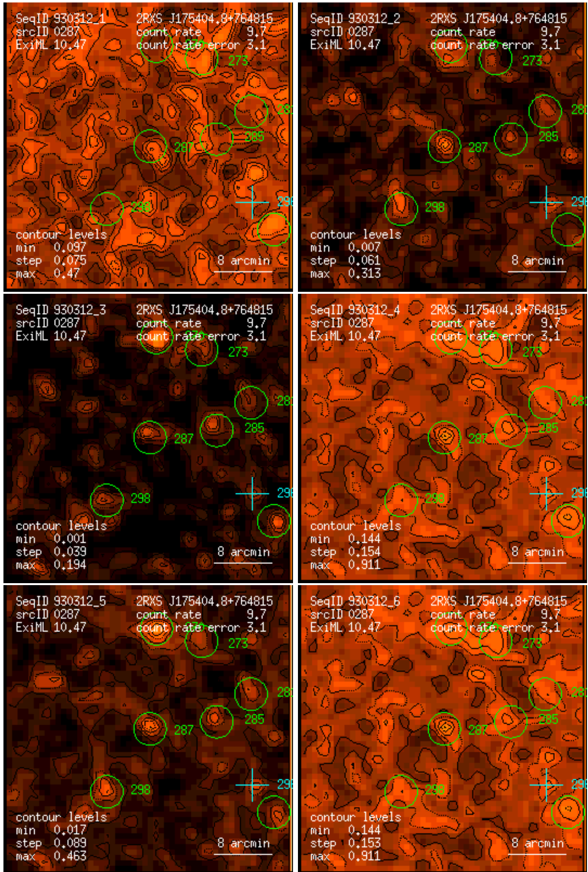
Figure 287: RASS 930312: detection 0287: band rate images, Gaussian filter: (1) PSPC channels 11 – 41, (2) 52 – 90, (3) 91 – 201, (4) 11 – 235, (5) 52 – 201, (6) 11 – 201. Broad band rates in counts/ks. Band rate contour levels in counts/ks/arcmin 2 .
