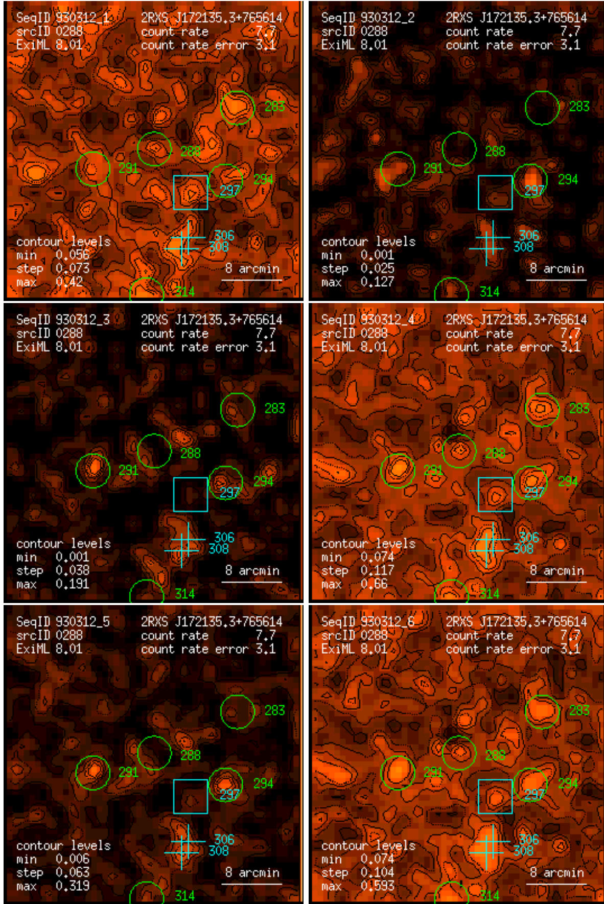
Figure 288: RASS 930312: detection 0288: band rate images, Gaussian filter: (1) PSPC channels 11 – 41, (2) 52 – 90, (3) 91 – 201, (4) 11 – 235, (5) 52 – 201, (6) 11 – 201. Broad band rates in counts/ks. Band rate contour levels in counts/ks/arcmin 2 .
