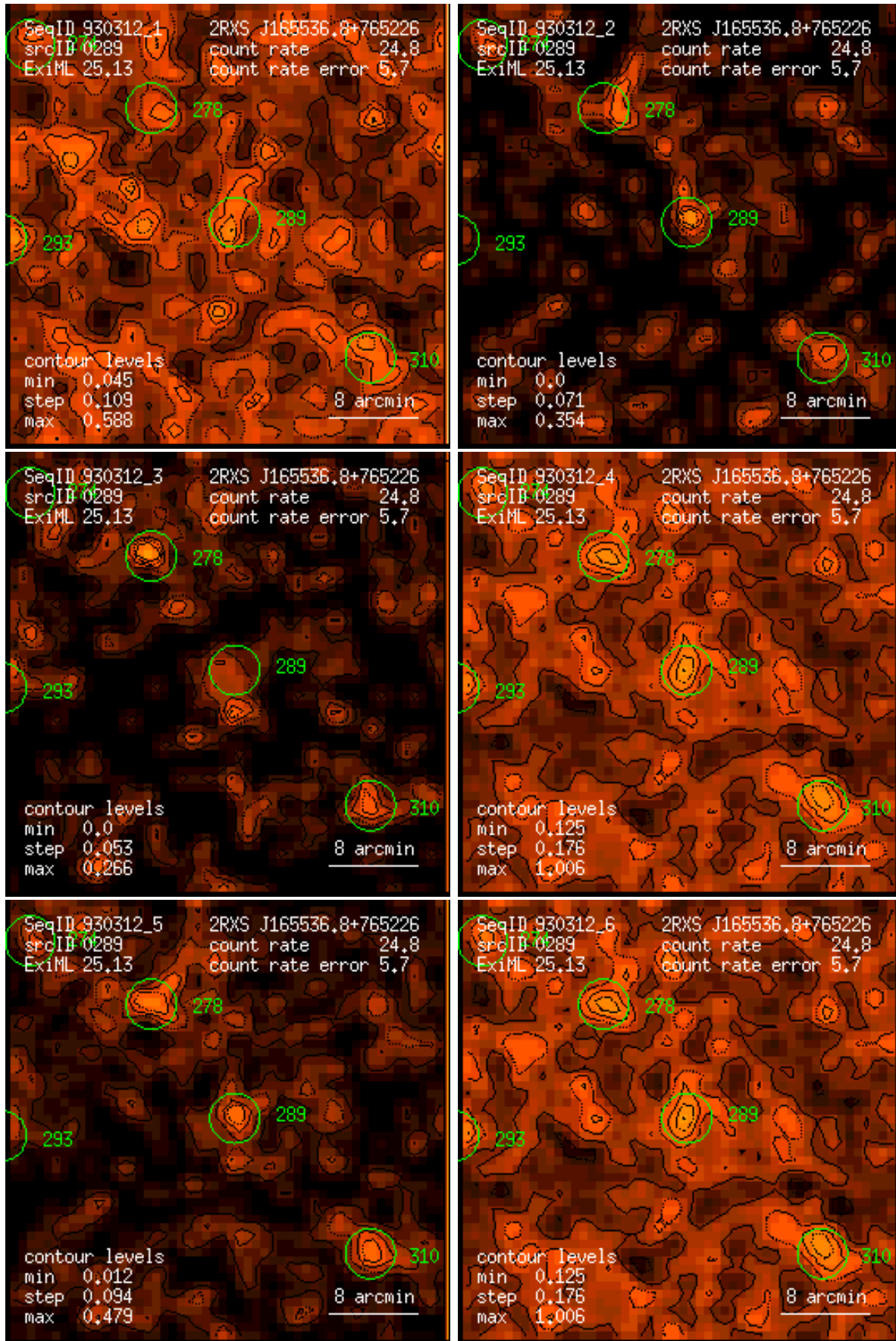
Figure 289: RASS 930312: detection 0289: band rate images, Gaussian filter: (1) PSPC channels 11 – 41, (2) 52 – 90, (3) 91 – 201, (4) 11 – 235, (5) 52 – 201, (6) 11 – 201. Broad band rates in counts/ks. Band rate contour levels in counts/ks/arcmin 2 .
