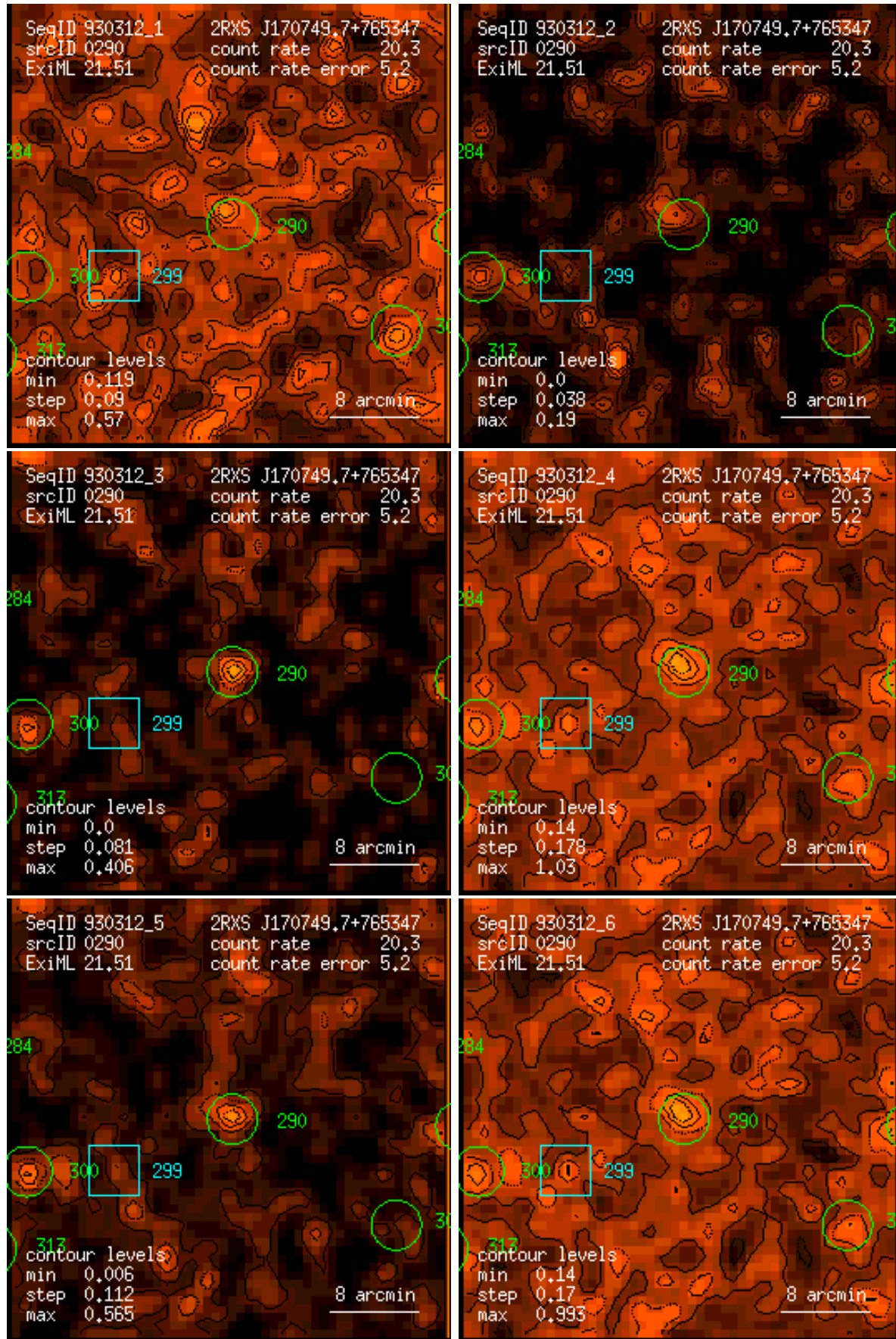
Figure 290: RASS 930312: detection 0290: band rate images, Gaussian filter: (1) PSPC channels 11 – 41, (2) 52 – 90, (3) 91 – 201, (4) 11 – 235, (5) 52 – 201, (6) 11 – 201. Broad band rates in counts/ks. Band rate contour levels in counts/ks/arcmin 2 .
