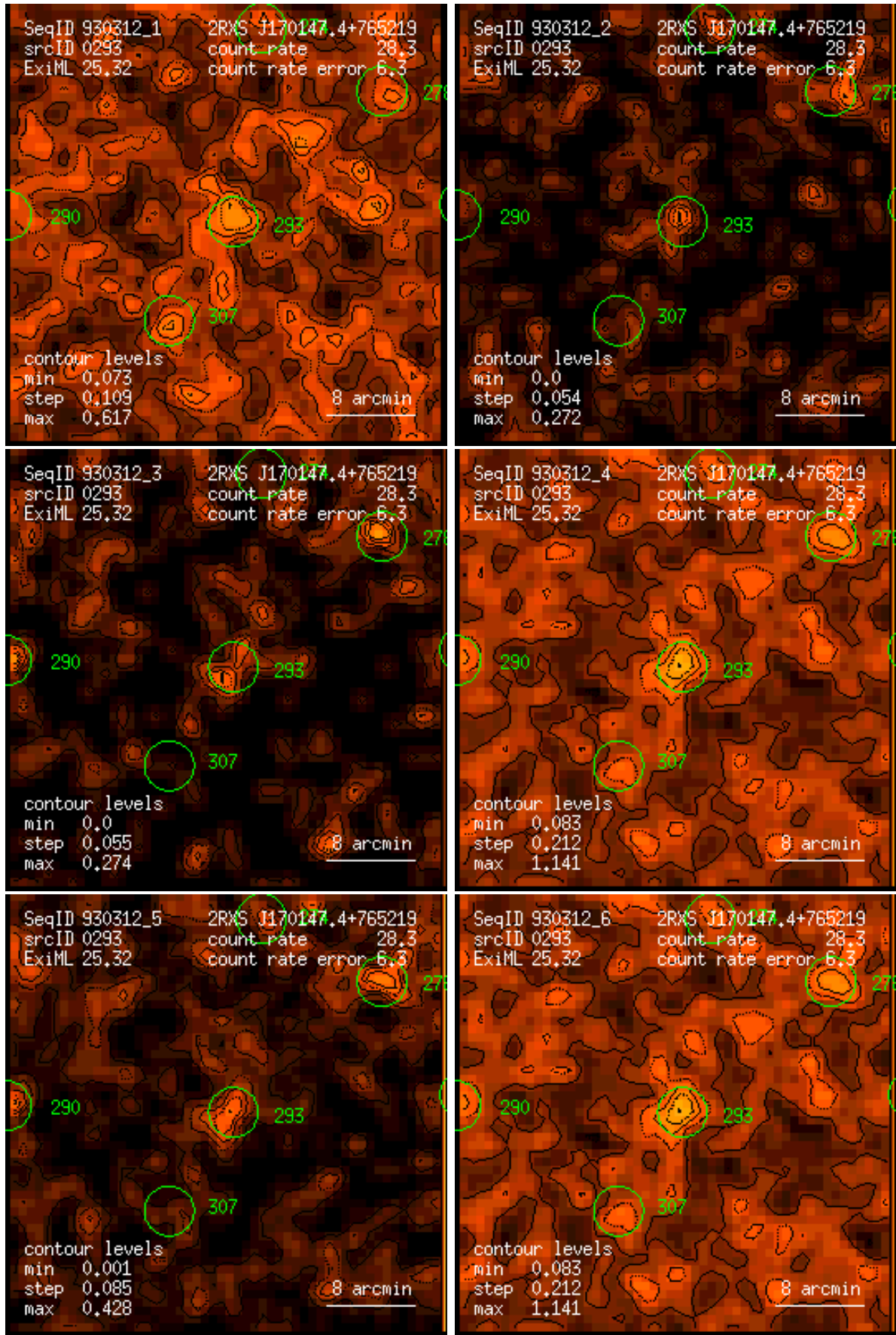
Figure 293: RASS 930312: detection 0293: band rate images, Gaussian filter: (1) PSPC channels 11 – 41, (2) 52 – 90, (3) 91 – 201, (4) 11 – 235, (5) 52 – 201, (6) 11 – 201. Broad band rates in counts/ks. Band rate contour levels in counts/ks/arcmin 2 .
