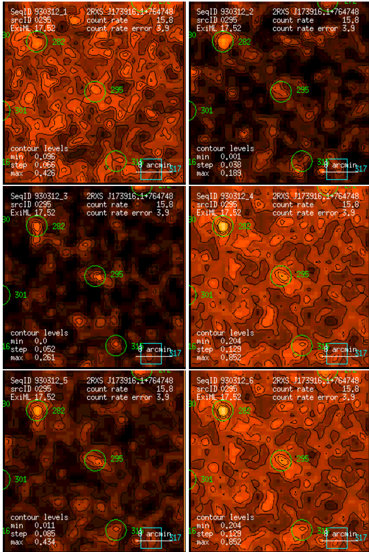
Figure 295: RASS 930312: detection 0295: band rate images, Gaussian filter: (1) PSPC channels 11 – 41, (2) 52 – 90, (3) 91 – 201, (4) 11 – 235, (5) 52 – 201, (6) 11 – 201. Broad band rates in counts/ks. Band rate contour levels in counts/ks/arcmin 2 .
