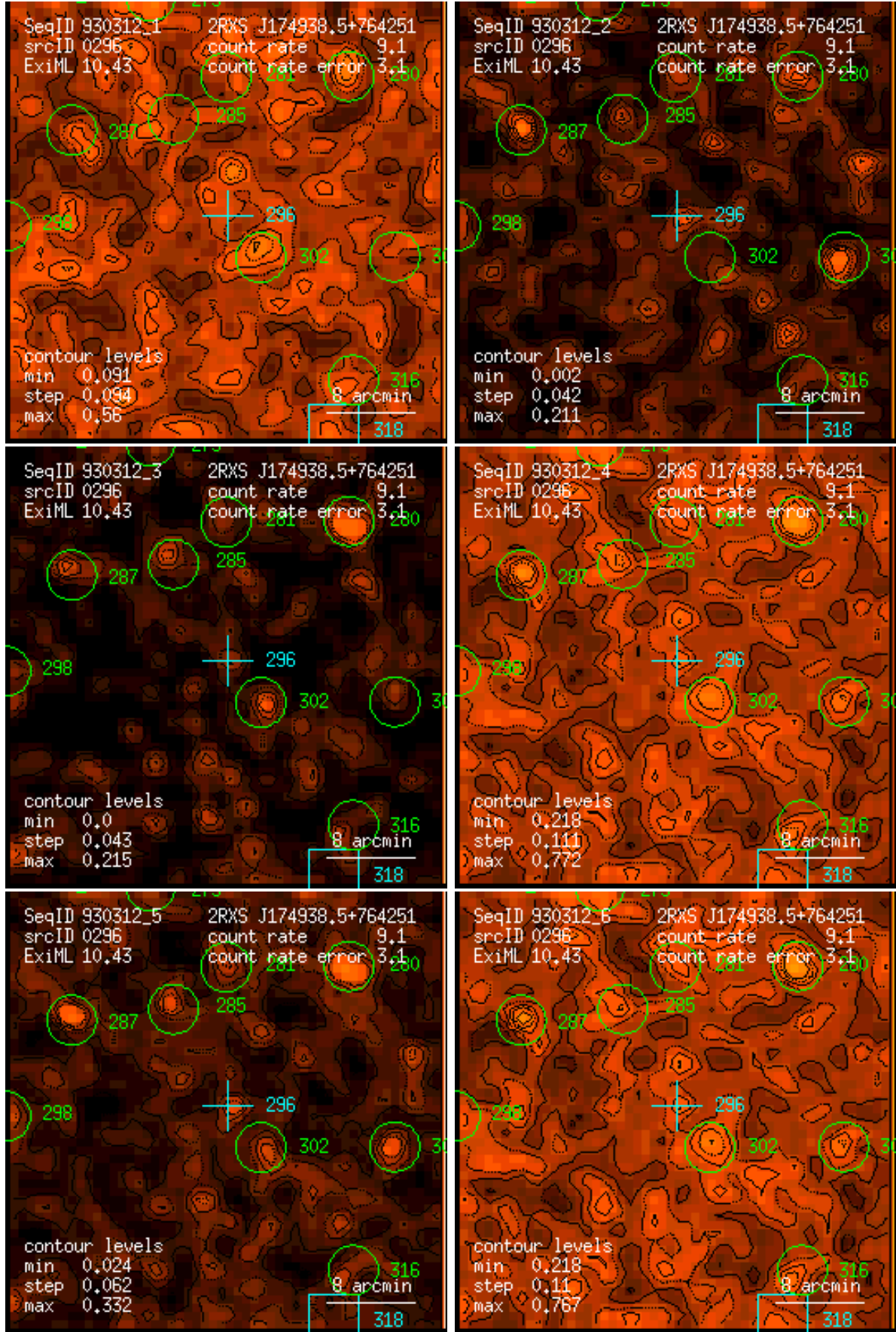
Figure 296: RASS 930312: detection 0296: band rate images, Gaussian filter: (1) PSPC channels 11 – 41, (2) 52 – 90, (3) 91 – 201, (4) 11 – 235, (5) 52 – 201, (6) 11 – 201. Broad band rates in counts/ks. Band rate contour levels in counts/ks/arcmin 2 .
