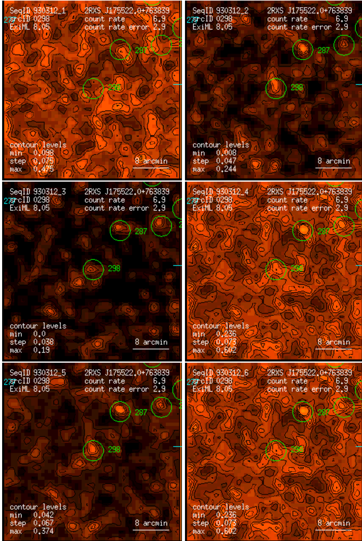
Figure 298: RASS 930312: detection 0298: band rate images, Gaussian filter: (1) PSPC channels 11 – 41, (2) 52 – 90, (3) 91 – 201, (4) 11 – 235, (5) 52 – 201, (6) 11 – 201. Broad band rates in counts/ks. Band rate contour levels in counts/ks/arcmin 2 .
