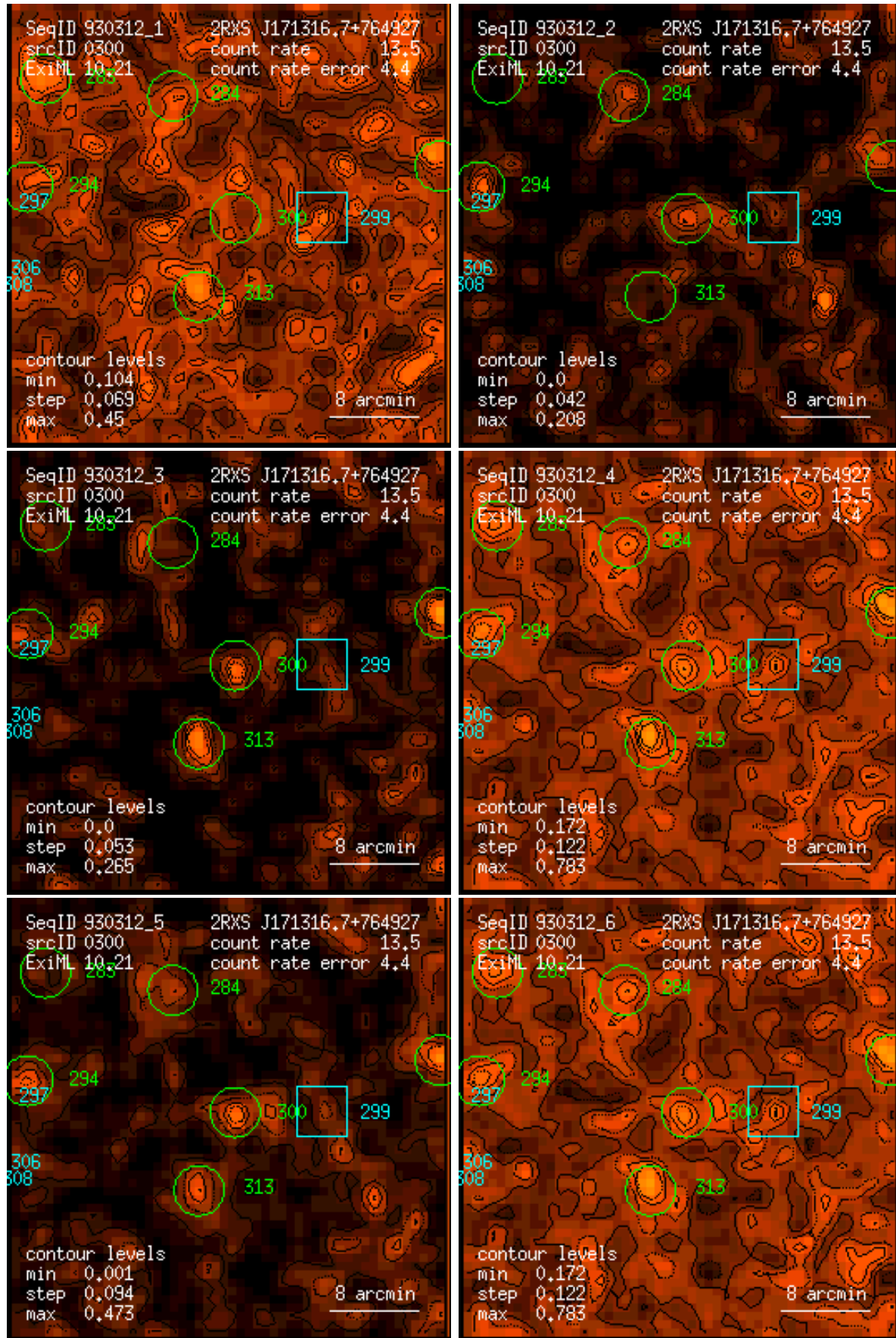
Figure 300: RASS 930312: detection 0300: band rate images, Gaussian filter: (1) PSPC channels 11 – 41, (2) 52 – 90, (3) 91 – 201, (4) 11 – 235, (5) 52 – 201, (6) 11 – 201. Broad band rates in counts/ks. Band rate contour levels in counts/ks/arcmin 2 .
