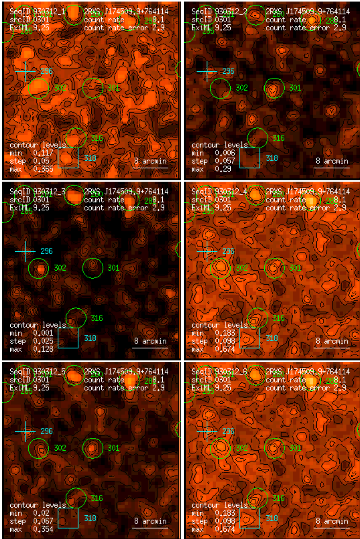
Figure 301: RASS 930312: detection 0301: band rate images, Gaussian filter: (1) PSPC channels 11 – 41, (2) 52 – 90, (3) 91 – 201, (4) 11 – 235, (5) 52 – 201, (6) 11 – 201. Broad band rates in counts/ks. Band rate contour levels in counts/ks/arcmin 2 .
