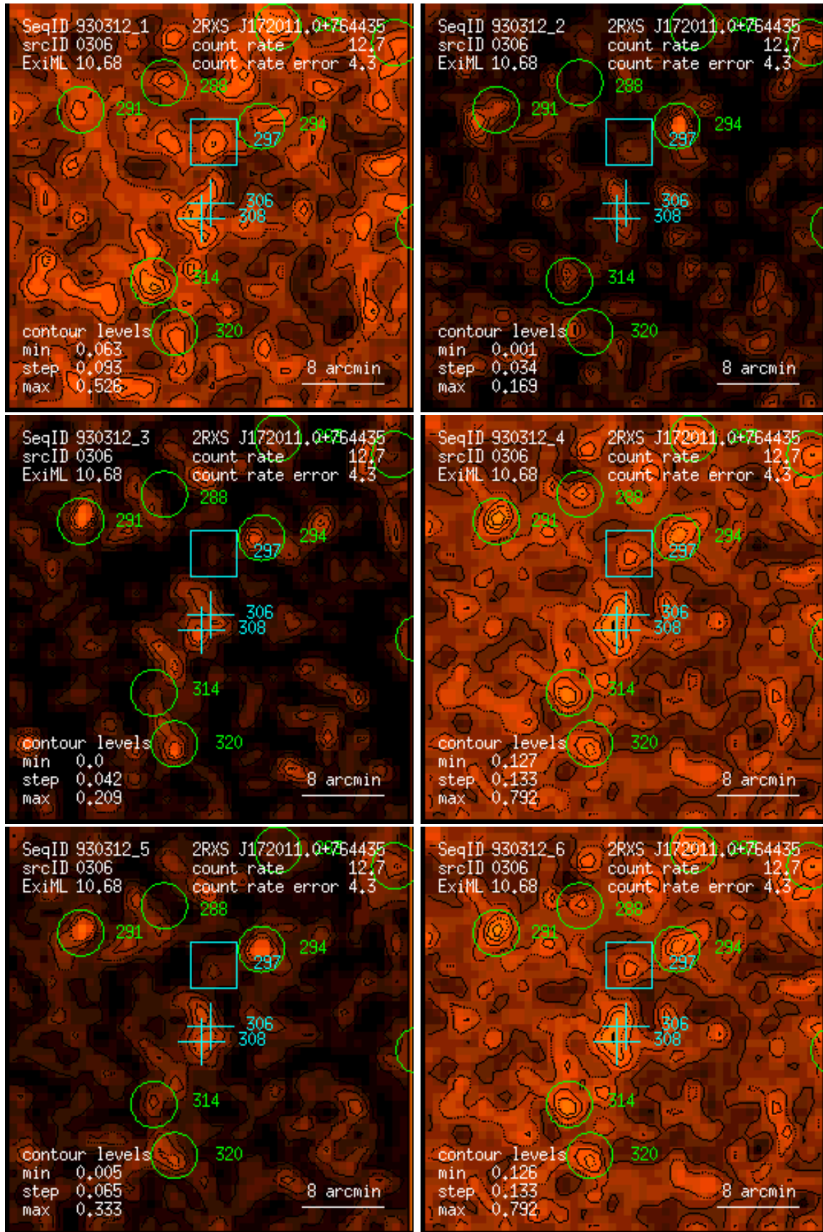
Figure 306: RASS 930312: detection 0306: band rate images, Gaussian filter: (1) PSPC channels 11 – 41, (2) 52 – 90, (3) 91 – 201, (4) 11 – 235, (5) 52 – 201, (6) 11 – 201. Broad band rates in counts/ks. Band rate contour levels in counts/ks/arcmin 2 .
