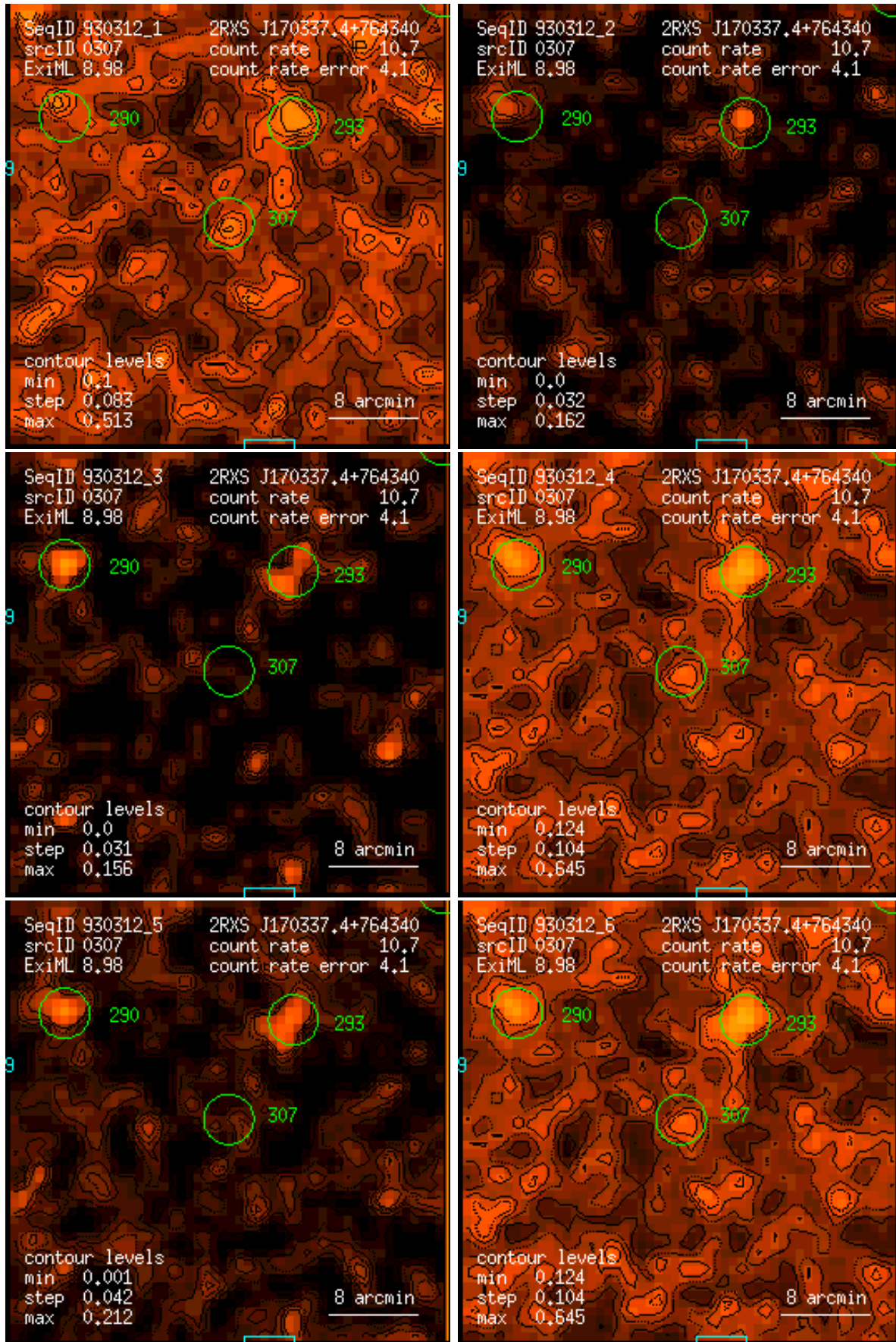
Figure 307: RASS 930312: detection 0307: band rate images, Gaussian filter: (1) PSPC channels 11 – 41, (2) 52 – 90, (3) 91 – 201, (4) 11 – 235, (5) 52 – 201, (6) 11 – 201. Broad band rates in counts/ks. Band rate contour levels in counts/ks/arcmin 2 .
