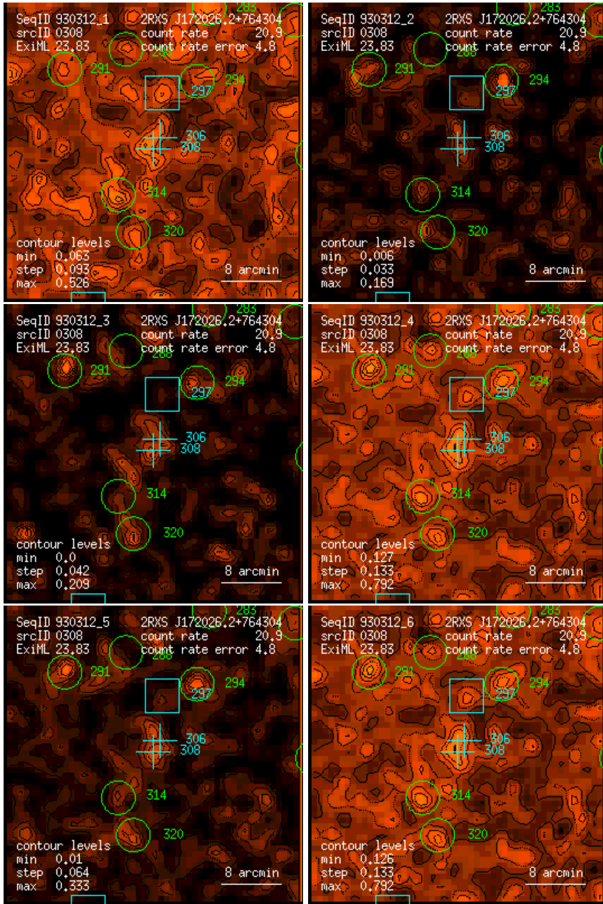
Figure 308: RASS 930312: detection 0308: band rate images, Gaussian filter: (1) PSPC channels 11 – 41, (2) 52 – 90, (3) 91 – 201, (4) 11 – 235, (5) 52 – 201, (6) 11 – 201. Broad band rates in counts/ks. Band rate contour levels in counts/ks/arcmin 2 .
