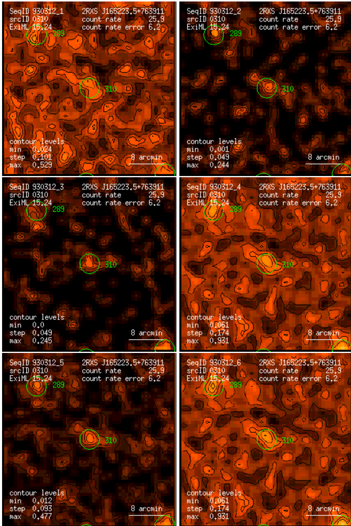
Figure 310: RASS 930312: detection 0310: band rate images, Gaussian filter: (1) PSPC channels 11 – 41, (2) 52 – 90, (3) 91 – 201, (4) 11 – 235, (5) 52 – 201, (6) 11 – 201. Broad band rates in counts/ks. Band rate contour levels in counts/ks/arcmin 2 .
