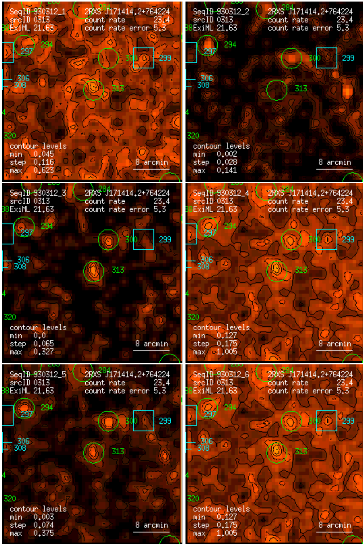
Figure 313: RASS 930312: detection 0313: band rate images, Gaussian filter: (1) PSPC channels 11 – 41, (2) 52 – 90, (3) 91 – 201, (4) 11 – 235, (5) 52 – 201, (6) 11 – 201. Broad band rates in counts/ks. Band rate contour levels in counts/ks/arcmin 2 .
