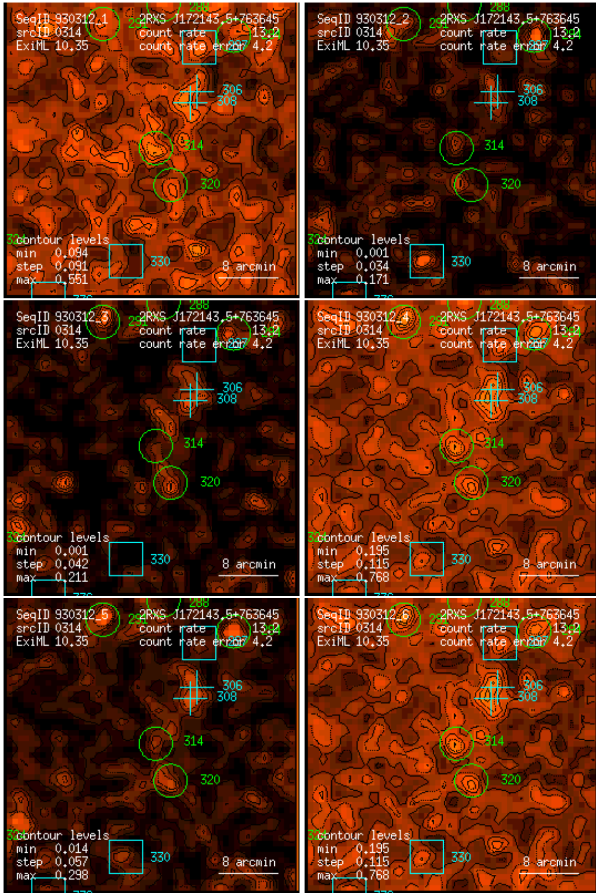
Figure 314: RASS 930312: detection 0314: band rate images, Gaussian filter: (1) PSPC channels 11 – 41, (2) 52 – 90, (3) 91 – 201, (4) 11 – 235, (5) 52 – 201, (6) 11 – 201. Broad band rates in counts/ks. Band rate contour levels in counts/ks/arcmin 2 .
