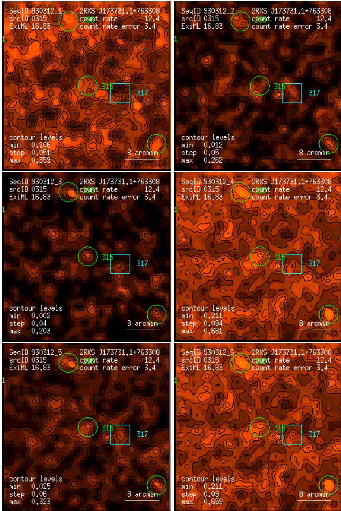
Figure 315: RASS 930312: detection 0315: band rate images, Gaussian filter: (1) PSPC channels 11 – 41, (2) 52 – 90, (3) 91 – 201, (4) 11 – 235, (5) 52 – 201, (6) 11 – 201. Broad band rates in counts/ks. Band rate contour levels in counts/ks/arcmin 2 .
