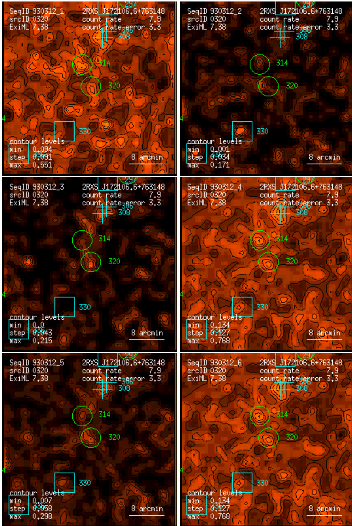
Figure 320: RASS 930312: detection 0320: band rate images, Gaussian filter: (1) PSPC channels 11 – 41, (2) 52 – 90, (3) 91 – 201, (4) 11 – 235, (5) 52 – 201, (6) 11 – 201. Broad band rates in counts/ks. Band rate contour levels in counts/ks/arcmin 2 .
