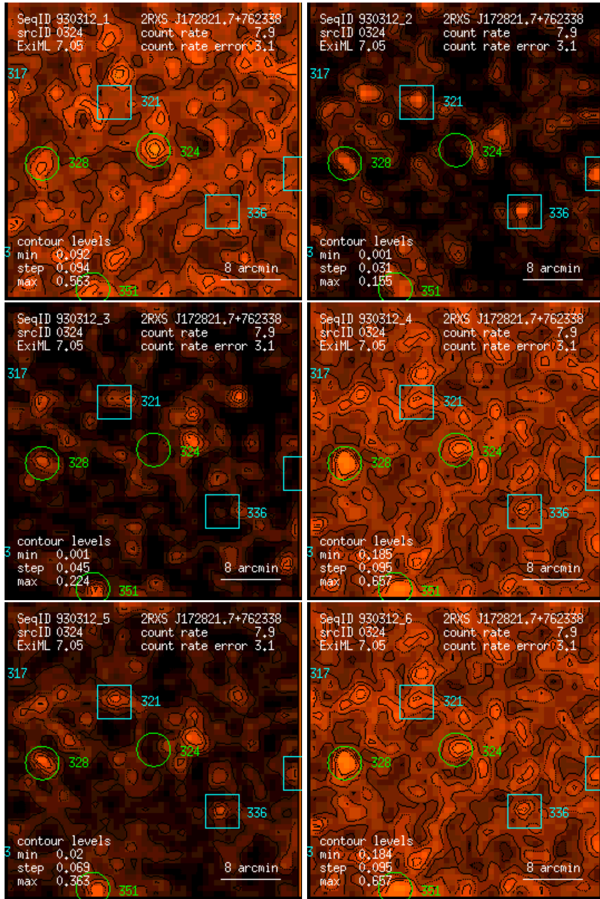
Figure 324: RASS 930312: detection 0324: band rate images, Gaussian filter: (1) PSPC channels 11 – 41, (2) 52 – 90, (3) 91 – 201, (4) 11 – 235, (5) 52 – 201, (6) 11 – 201. Broad band rates in counts/ks. Band rate contour levels in counts/ks/arcmin 2 .
