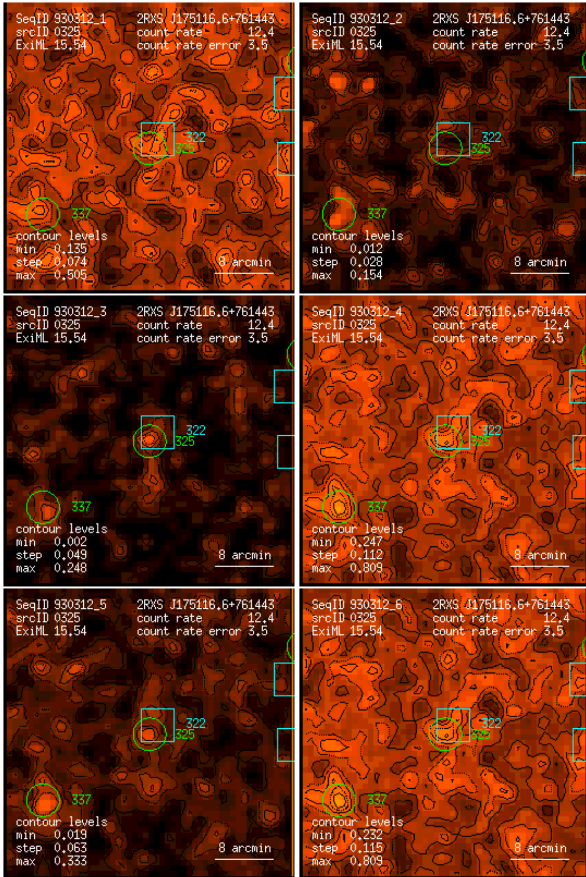
Figure 325: RASS 930312: detection 0325: band rate images, Gaussian filter: (1) PSPC channels 11 – 41, (2) 52 – 90, (3) 91 – 201, (4) 11 – 235, (5) 52 – 201, (6) 11 – 201. Broad band rates in counts/ks. Band rate contour levels in counts/ks/arcmin 2 .
