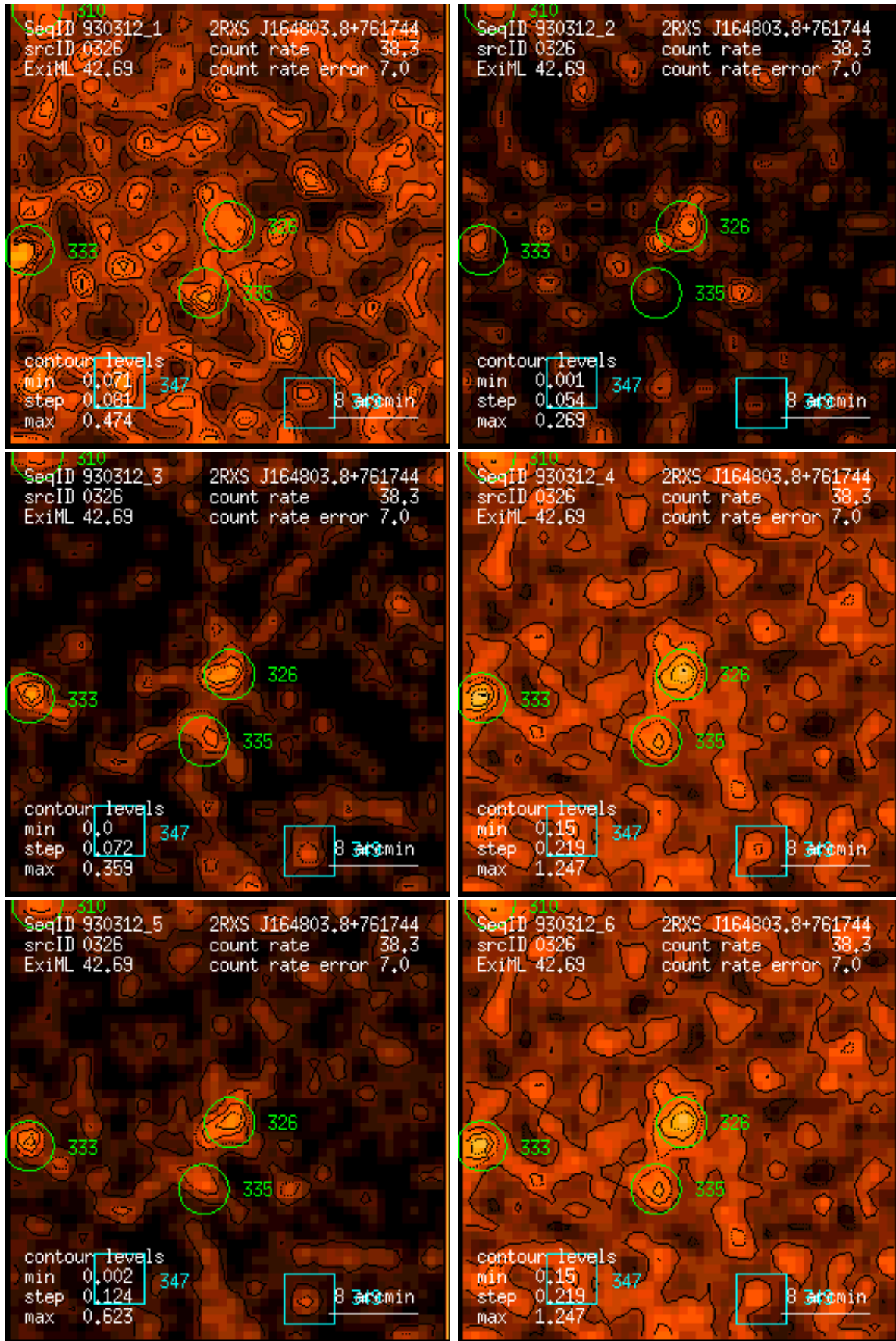
Figure 326: RASS 930312: detection 0326: band rate images, Gaussian filter: (1) PSPC channels 11 – 41, (2) 52 – 90, (3) 91 – 201, (4) 11 – 235, (5) 52 – 201, (6) 11 – 201. Broad band rates in counts/ks. Band rate contour levels in counts/ks/arcmin 2 .
