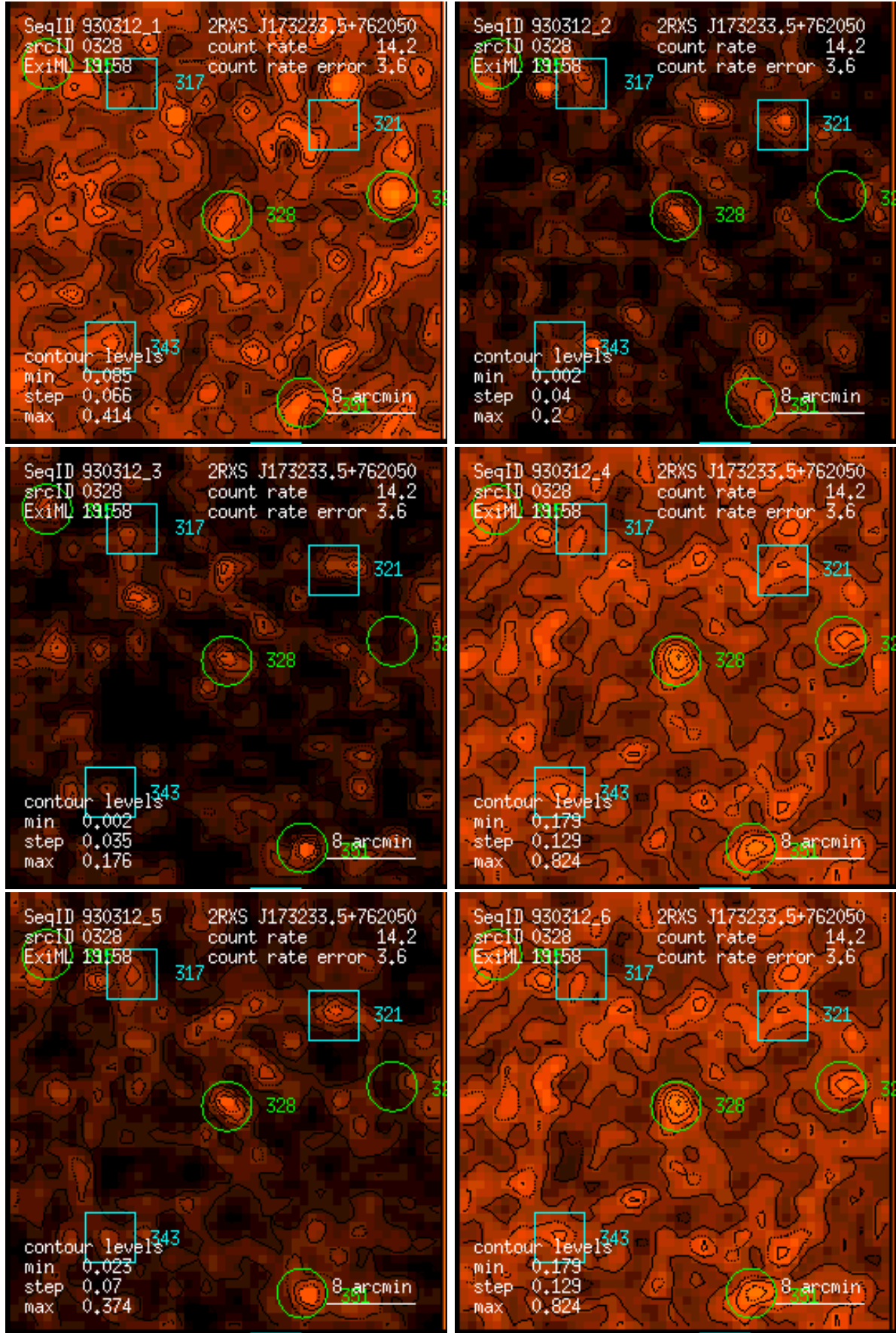
Figure 328: RASS 930312: detection 0328: band rate images, Gaussian filter: (1) PSPC channels 11 – 41, (2) 52 – 90, (3) 91 – 201, (4) 11 – 235, (5) 52 – 201, (6) 11 – 201. Broad band rates in counts/ks. Band rate contour levels in counts/ks/arcmin 2 .
