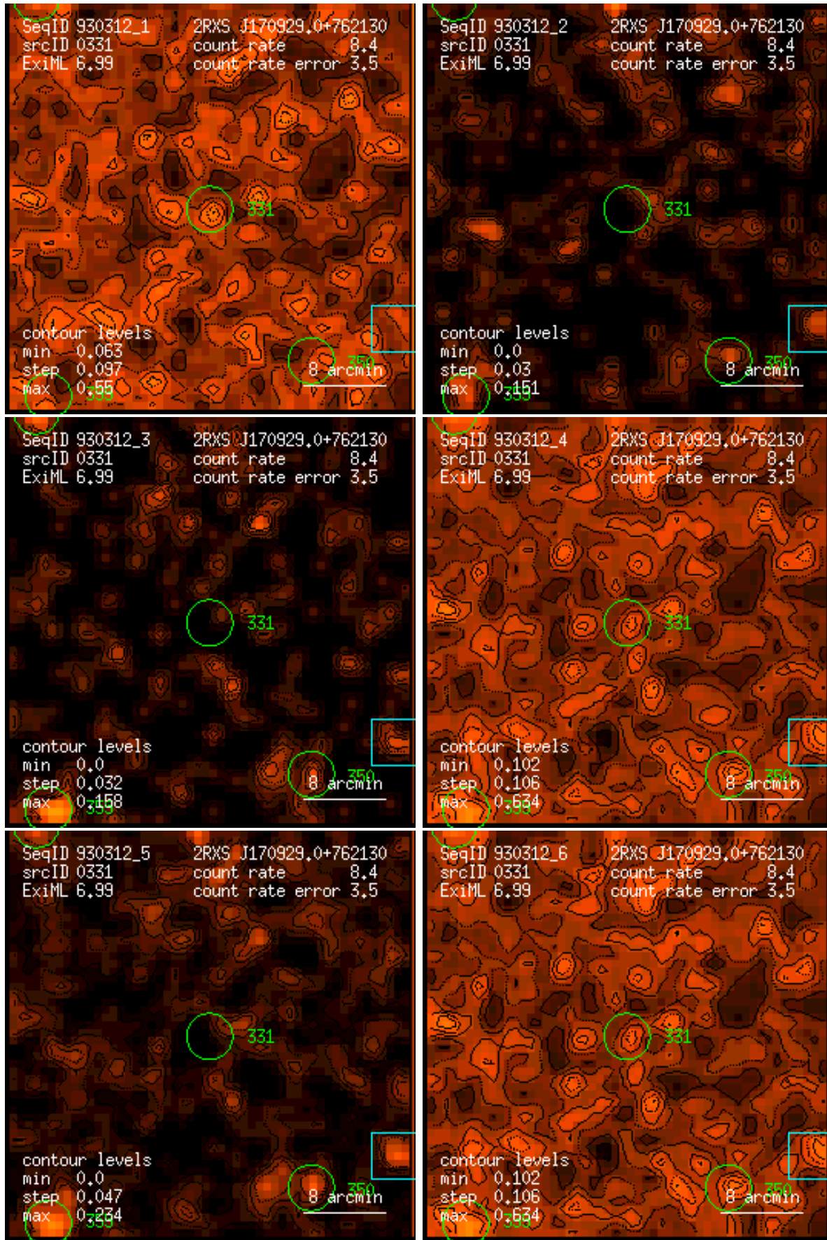
Figure 331: RASS 930312: detection 0331: band rate images, Gaussian filter: (1) PSPC channels 11 – 41, (2) 52 – 90, (3) 91 – 201, (4) 11 – 235, (5) 52 – 201, (6) 11 – 201. Broad band rates in counts/ks. Band rate contour levels in counts/ks/arcmin 2 .
