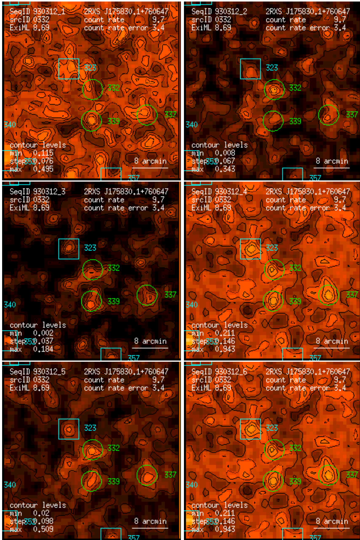
Figure 332: RASS 930312: detection 0332: band rate images, Gaussian filter: (1) PSPC channels 11 – 41, (2) 52 – 90, (3) 91 – 201, (4) 11 – 235, (5) 52 – 201, (6) 11 – 201. Broad band rates in counts/ks. Band rate contour levels in counts/ks/arcmin 2 .
