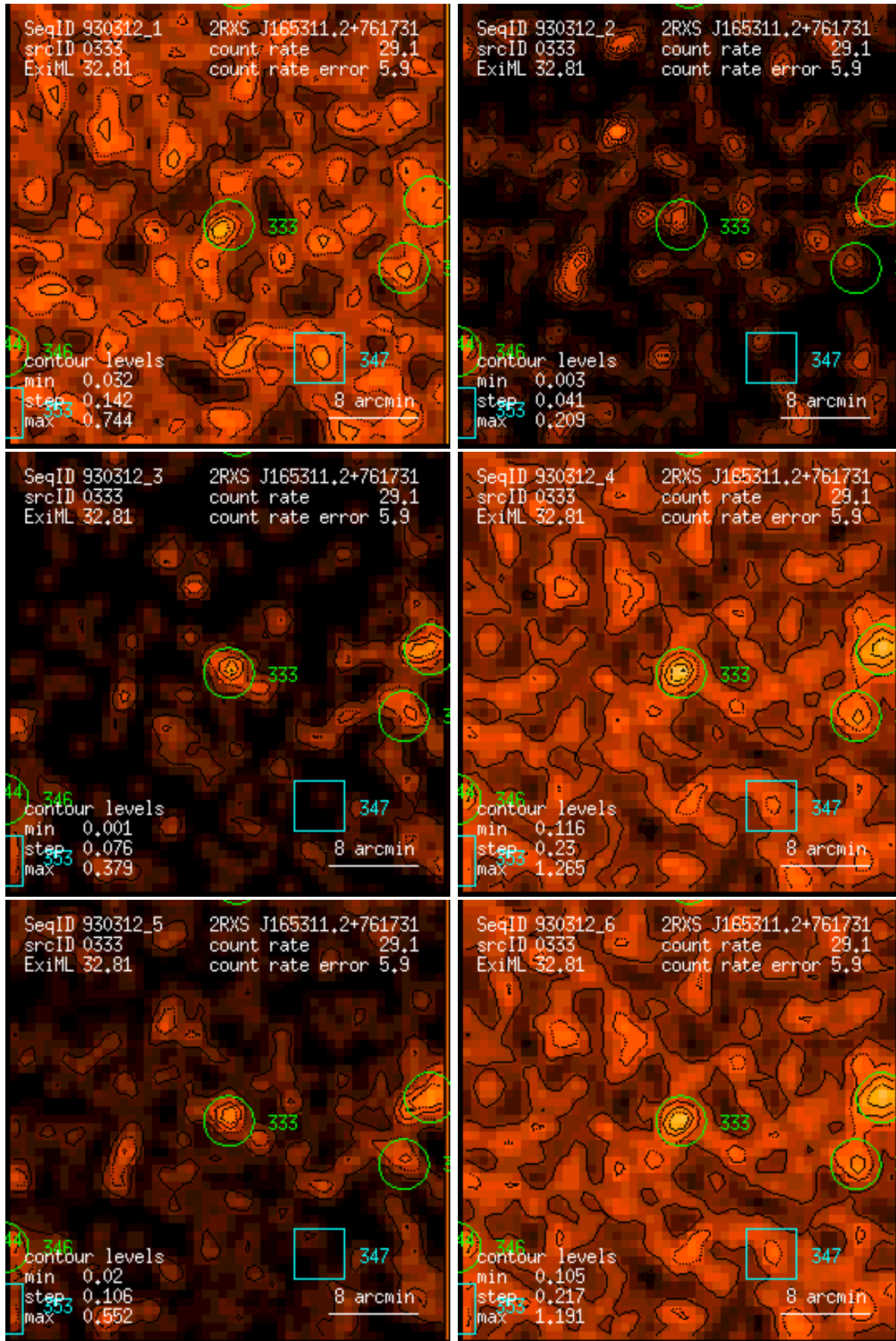
Figure 333: RASS 930312: detection 0333: band rate images, Gaussian filter: (1) PSPC channels 11 – 41, (2) 52 – 90, (3) 91 – 201, (4) 11 – 235, (5) 52 – 201, (6) 11 – 201. Broad band rates in counts/ks. Band rate contour levels in counts/ks/arcmin 2 .
