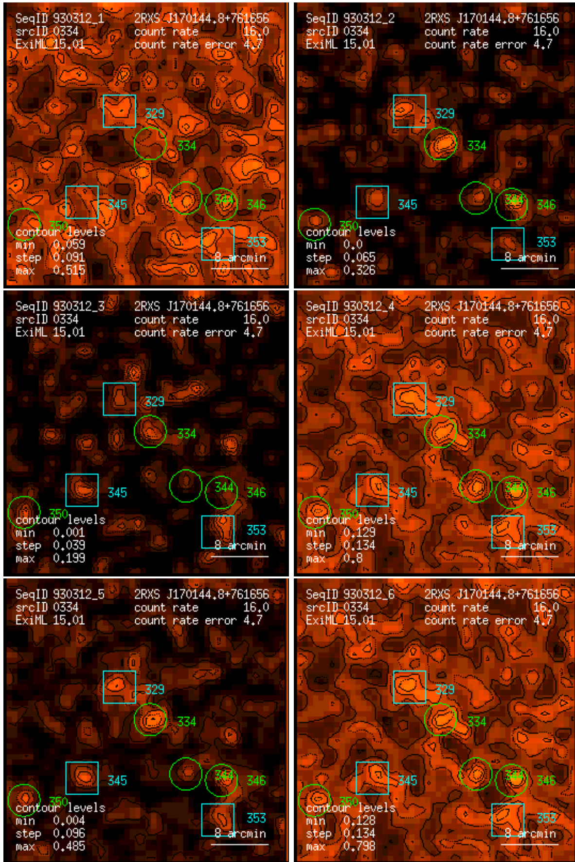
Figure 334: RASS 930312: detection 0334: band rate images, Gaussian filter: (1) PSPC channels 11 – 41, (2) 52 – 90, (3) 91 – 201, (4) 11 – 235, (5) 52 – 201, (6) 11 – 201. Broad band rates in counts/ks. Band rate contour levels in counts/ks/arcmin 2 .
