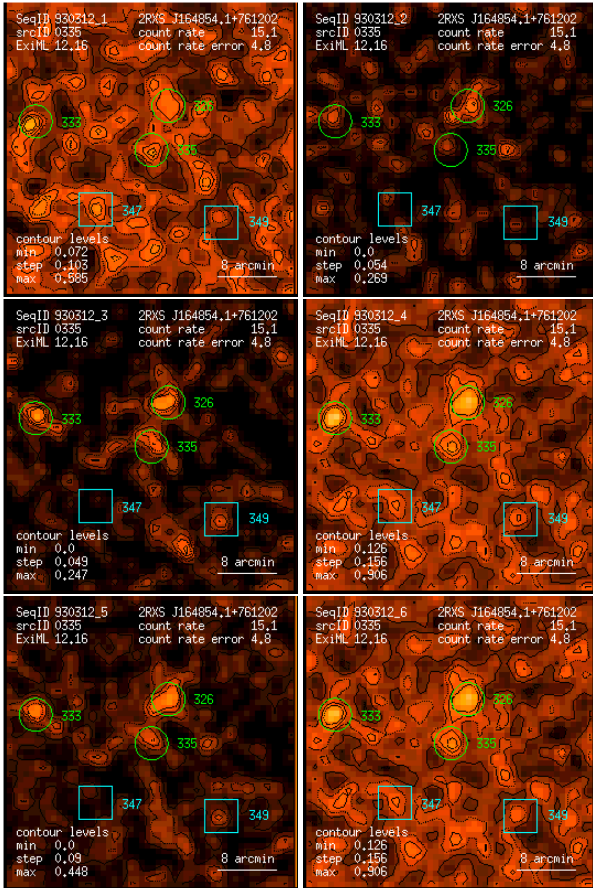
Figure 335: RASS 930312: detection 0335: band rate images, Gaussian filter: (1) PSPC channels 11 – 41, (2) 52 – 90, (3) 91 – 201, (4) 11 – 235, (5) 52 – 201, (6) 11 – 201. Broad band rates in counts/ks. Band rate contour levels in counts/ks/arcmin 2 .
