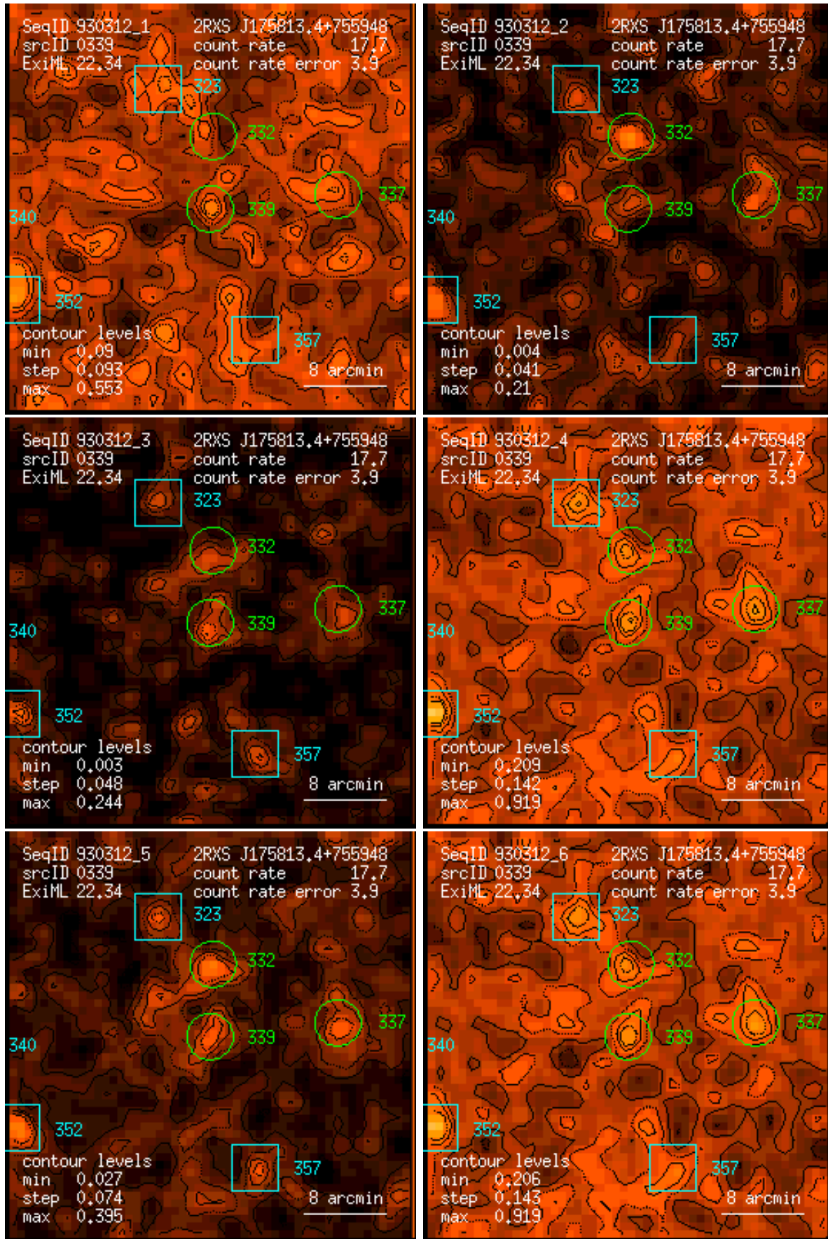
Figure 339: RASS 930312: detection 0339: band rate images, Gaussian filter: (1) PSPC channels 11 – 41, (2) 52 – 90, (3) 91 – 201, (4) 11 – 235, (5) 52 – 201, (6) 11 – 201. Broad band rates in counts/ks. Band rate contour levels in counts/ks/arcmin 2 .
