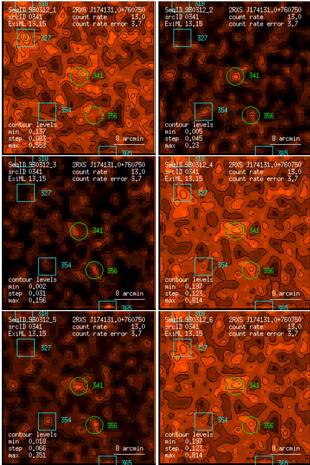
Figure 341: RASS 930312: detection 0341: band rate images, Gaussian filter: (1) PSPC channels 11 – 41, (2) 52 – 90, (3) 91 – 201, (4) 11 – 235, (5) 52 – 201, (6) 11 – 201. Broad band rates in counts/ks. Band rate contour levels in counts/ks/arcmin 2 .
