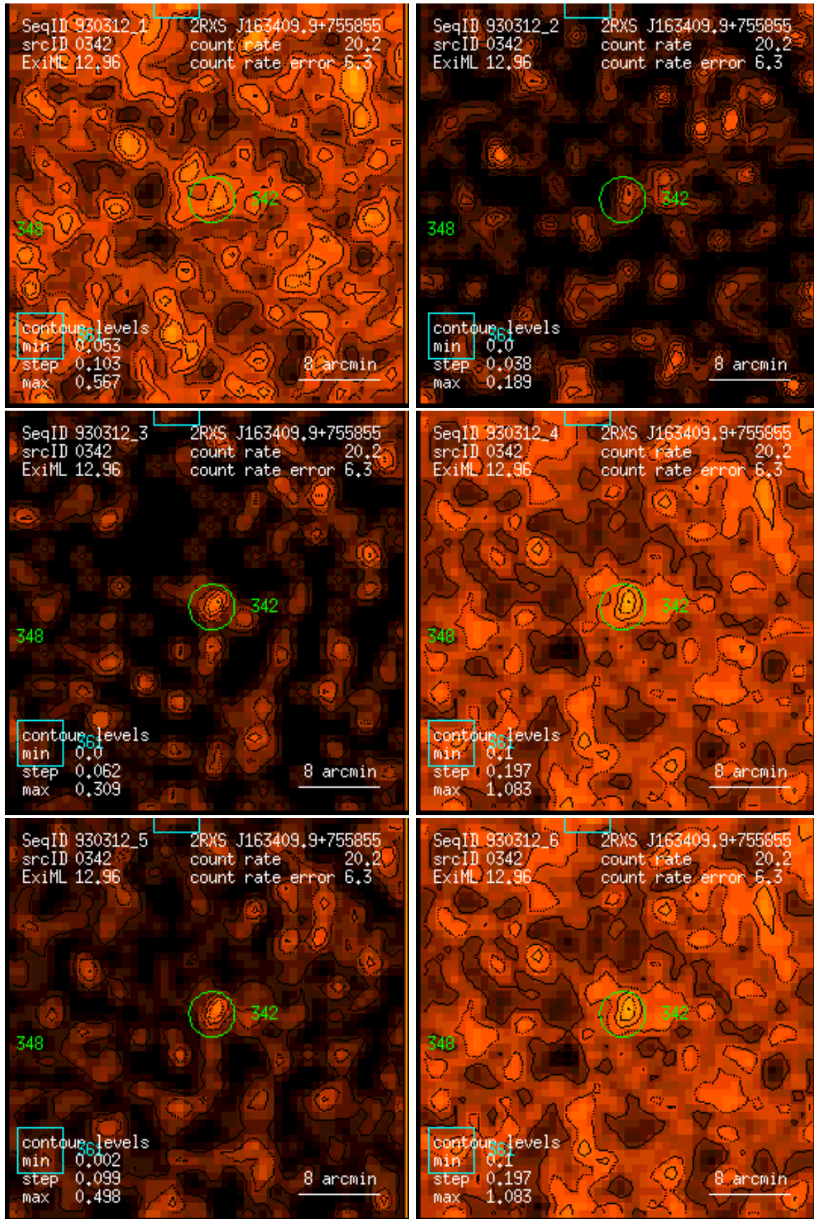
Figure 342: RASS 930312: detection 0342: band rate images, Gaussian filter: (1) PSPC channels 11 – 41, (2) 52 – 90, (3) 91 – 201, (4) 11 – 235, (5) 52 – 201, (6) 11 – 201. Broad band rates in counts/ks. Band rate contour levels in counts/ks/arcmin 2 .
