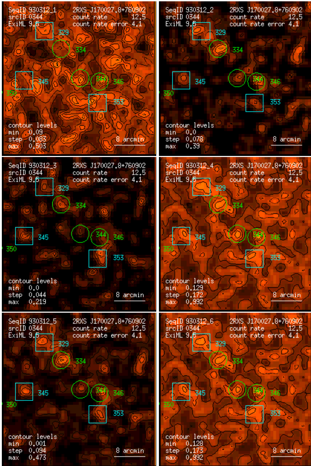
Figure 344: RASS 930312: detection 0344: band rate images, Gaussian filter: (1) PSPC channels 11 – 41, (2) 52 – 90, (3) 91 – 201, (4) 11 – 235, (5) 52 – 201, (6) 11 – 201. Broad band rates in counts/ks. Band rate contour levels in counts/ks/arcmin 2 .
