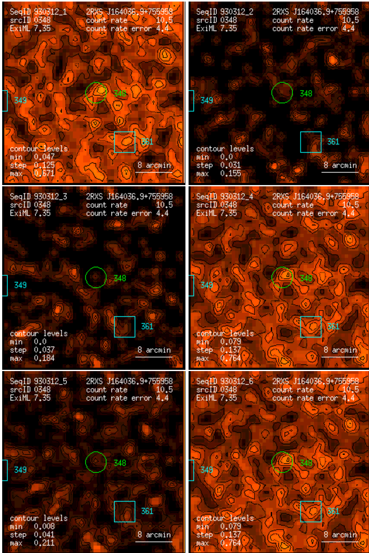
Figure 348: RASS 930312: detection 0348: band rate images, Gaussian filter: (1) PSPC channels 11 – 41, (2) 52 – 90, (3) 91 – 201, (4) 11 – 235, (5) 52 – 201, (6) 11 – 201. Broad band rates in counts/ks. Band rate contour levels in counts/ks/arcmin 2 .
