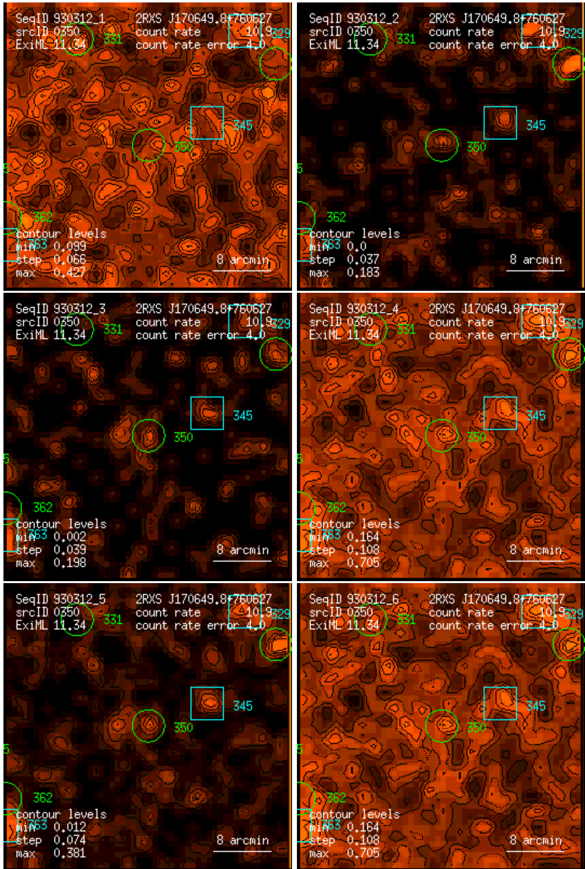
Figure 350: RASS 930312: detection 0350: band rate images, Gaussian filter: (1) PSPC channels 11 – 41, (2) 52 – 90, (3) 91 – 201, (4) 11 – 235, (5) 52 – 201, (6) 11 – 201. Broad band rates in counts/ks. Band rate contour levels in counts/ks/arcmin 2 .
