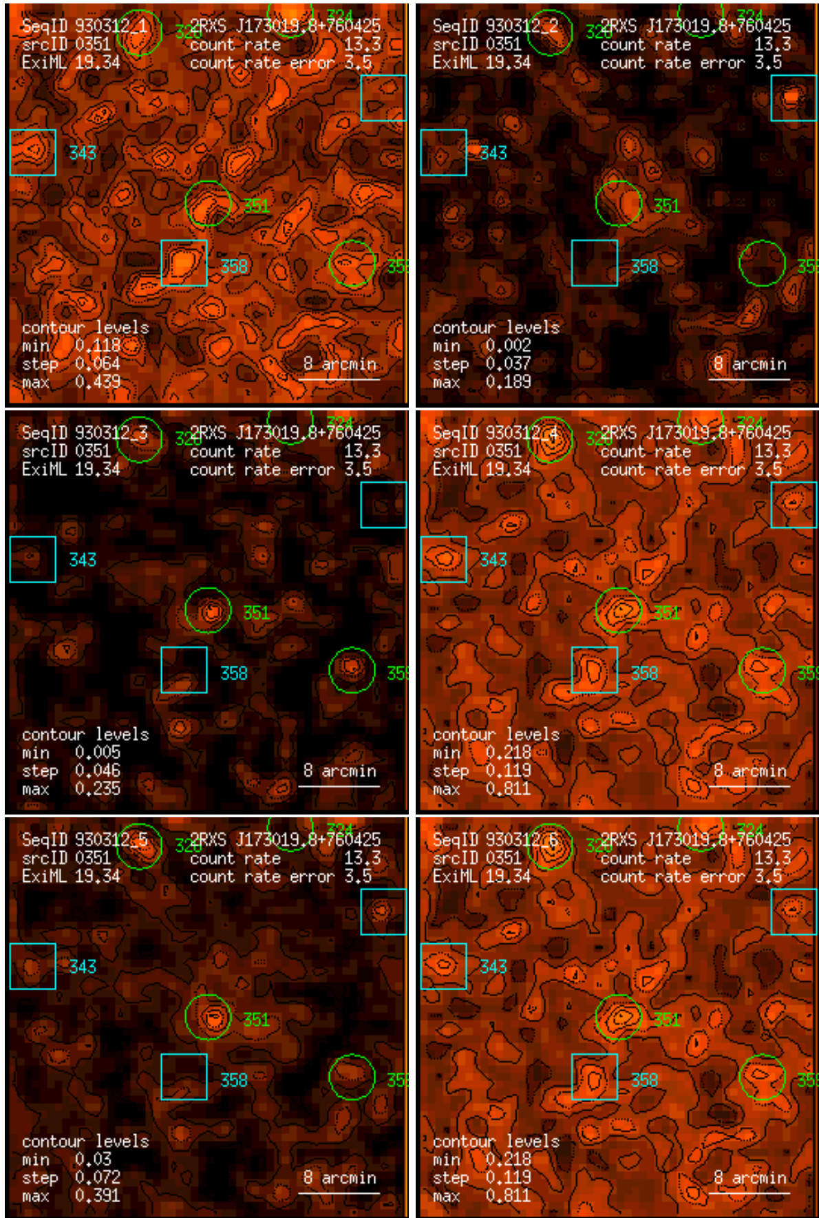
Figure 351: RASS 930312: detection 0351: band rate images, Gaussian filter: (1) PSPC channels 11 – 41, (2) 52 – 90, (3) 91 – 201, (4) 11 – 235, (5) 52 – 201, (6) 11 – 201. Broad band rates in counts/ks. Band rate contour levels in counts/ks/arcmin 2 .
