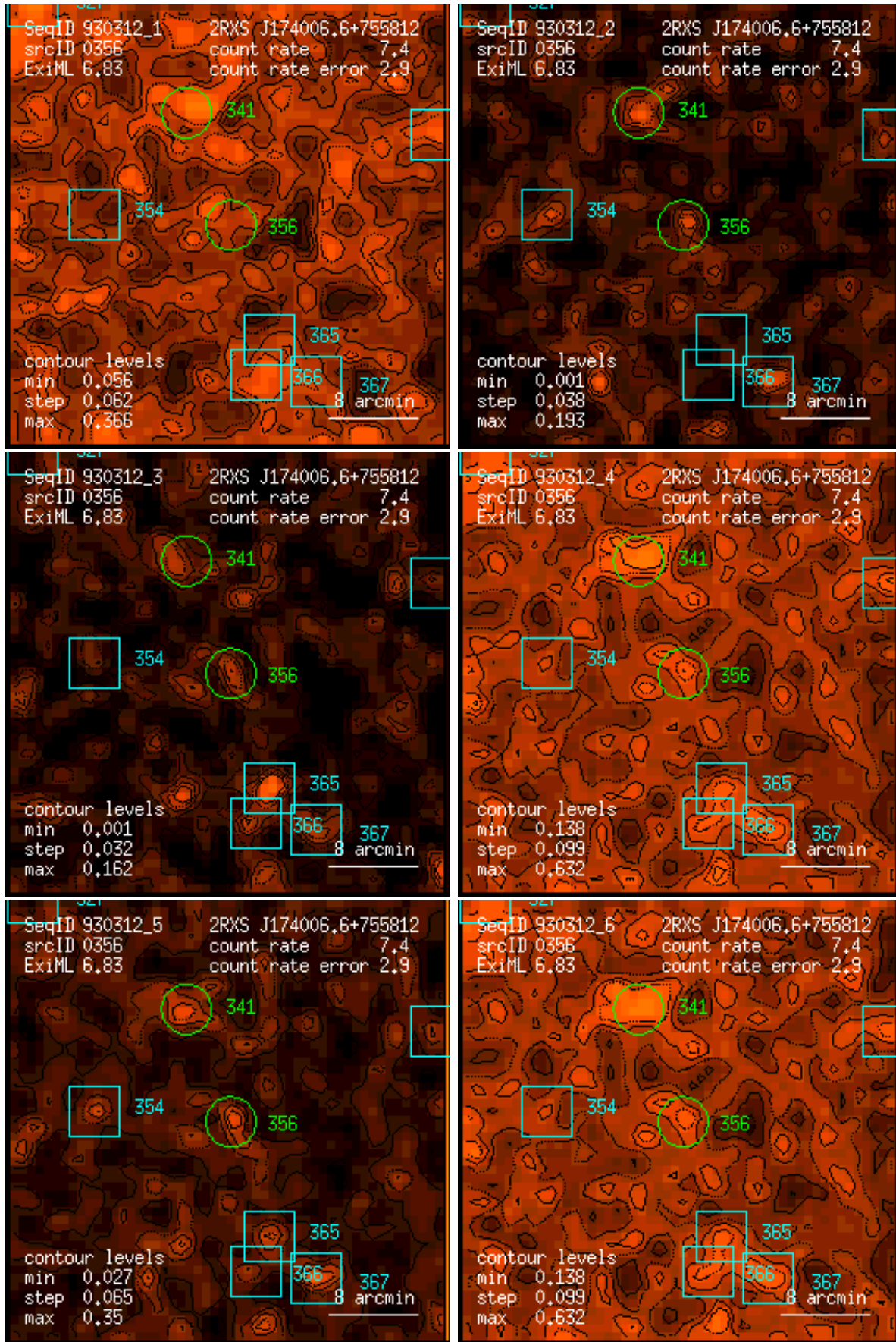
Figure 356: RASS 930312: detection 0356: band rate images, Gaussian filter: (1) PSPC channels 11 – 41, (2) 52 – 90, (3) 91 – 201, (4) 11 – 235, (5) 52 – 201, (6) 11 – 201. Broad band rates in counts/ks. Band rate contour levels in counts/ks/arcmin 2 .
