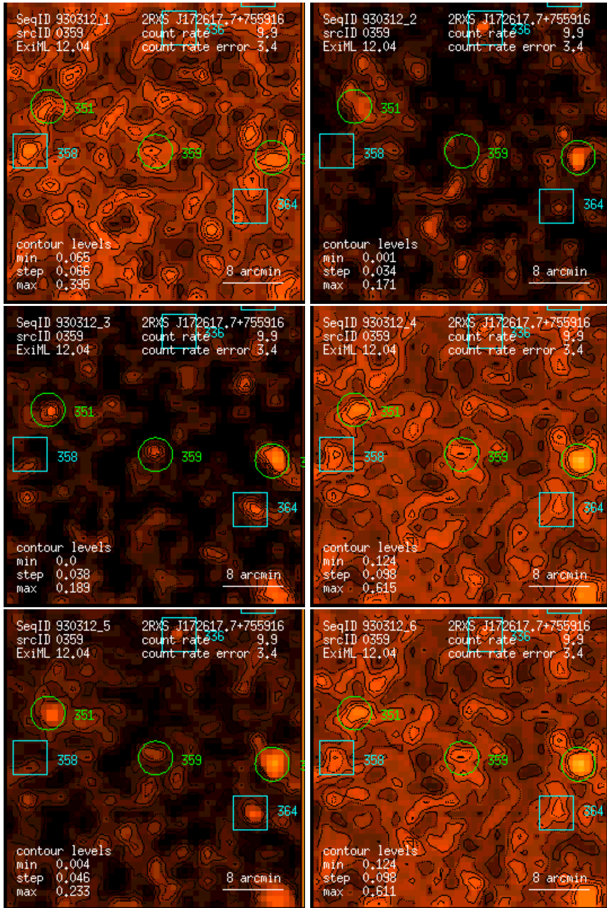
Figure 359: RASS 930312: detection 0359: band rate images, Gaussian filter: (1) PSPC channels 11 – 41, (2) 52 – 90, (3) 91 – 201, (4) 11 – 235, (5) 52 – 201, (6) 11 – 201. Broad band rates in counts/ks. Band rate contour levels in counts/ks/arcmin 2 .
