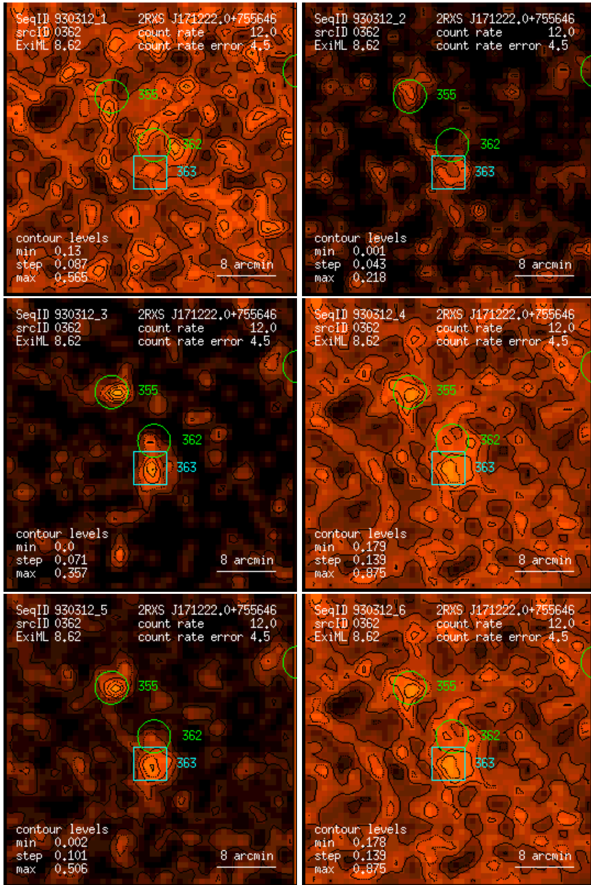
Figure 362: RASS 930312: detection 0362: band rate images, Gaussian filter: (1) PSPC channels 11 – 41, (2) 52 – 90, (3) 91 – 201, (4) 11 – 235, (5) 52 – 201, (6) 11 – 201. Broad band rates in counts/ks. Band rate contour levels in counts/ks/arcmin 2 .
