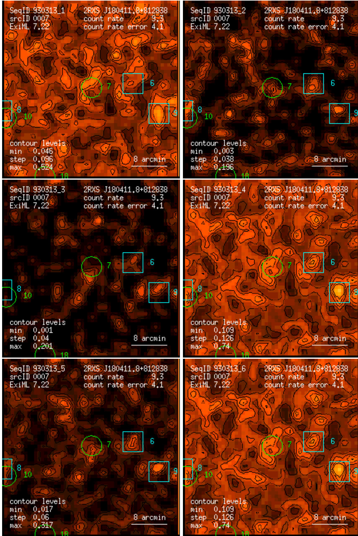
Figure 7: RASS 930313: detection 0007: band rate images, Gaussian filter: (1) PSPC channels 11 – 41, (2) 52 – 90, (3) 91 – 201, (4) 11 – 235, (5) 52 – 201, (6) 11 – 201. Broad band rates in counts/ks. Band rate contour levels in counts/ks/arcmin 2 .
