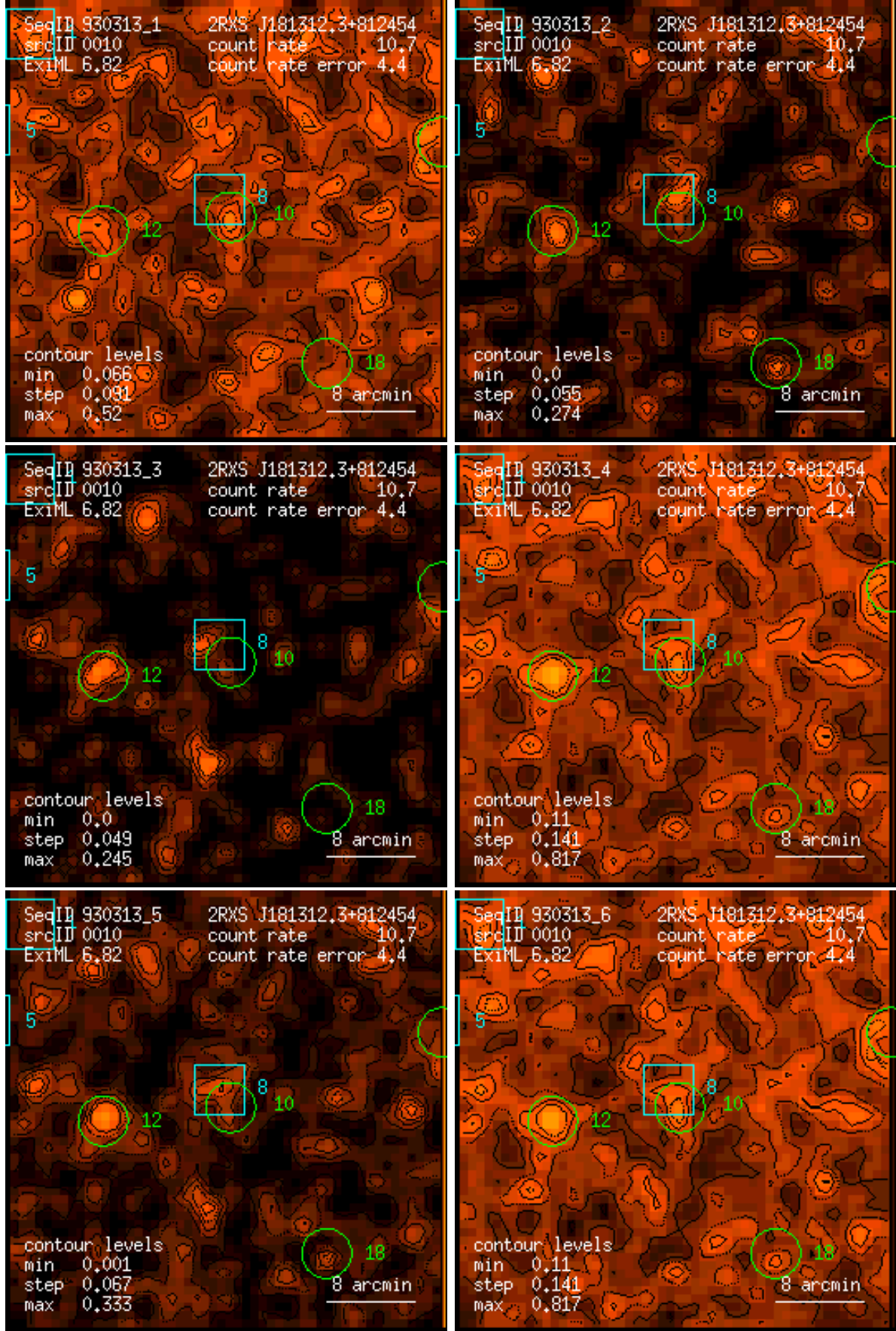
Figure 10: RASS 930313: detection 0010: band rate images, Gaussian filter: (1) PSPC channels 11 – 41, (2) 52 – 90, (3) 91 – 201, (4) 11 – 235, (5) 52 – 201, (6) 11 – 201. Broad band rates in counts/ks. Band rate contour levels in counts/ks/arcmin 2 .
