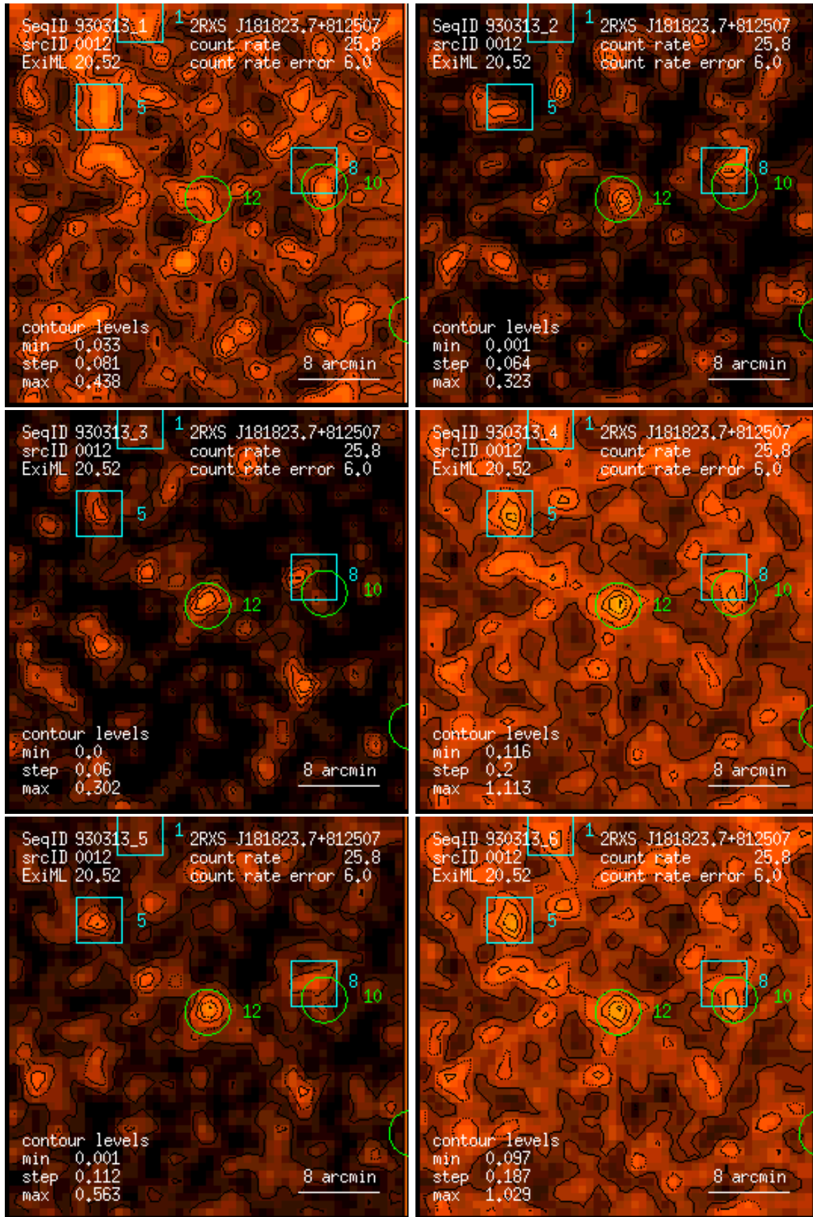
Figure 12: RASS 930313: detection 0012: band rate images, Gaussian filter: (1) PSPC channels 11 – 41, (2) 52 – 90, (3) 91 – 201, (4) 11 – 235, (5) 52 – 201, (6) 11 – 201. Broad band rates in counts/ks. Band rate contour levels in counts/ks/arcmin 2 .
