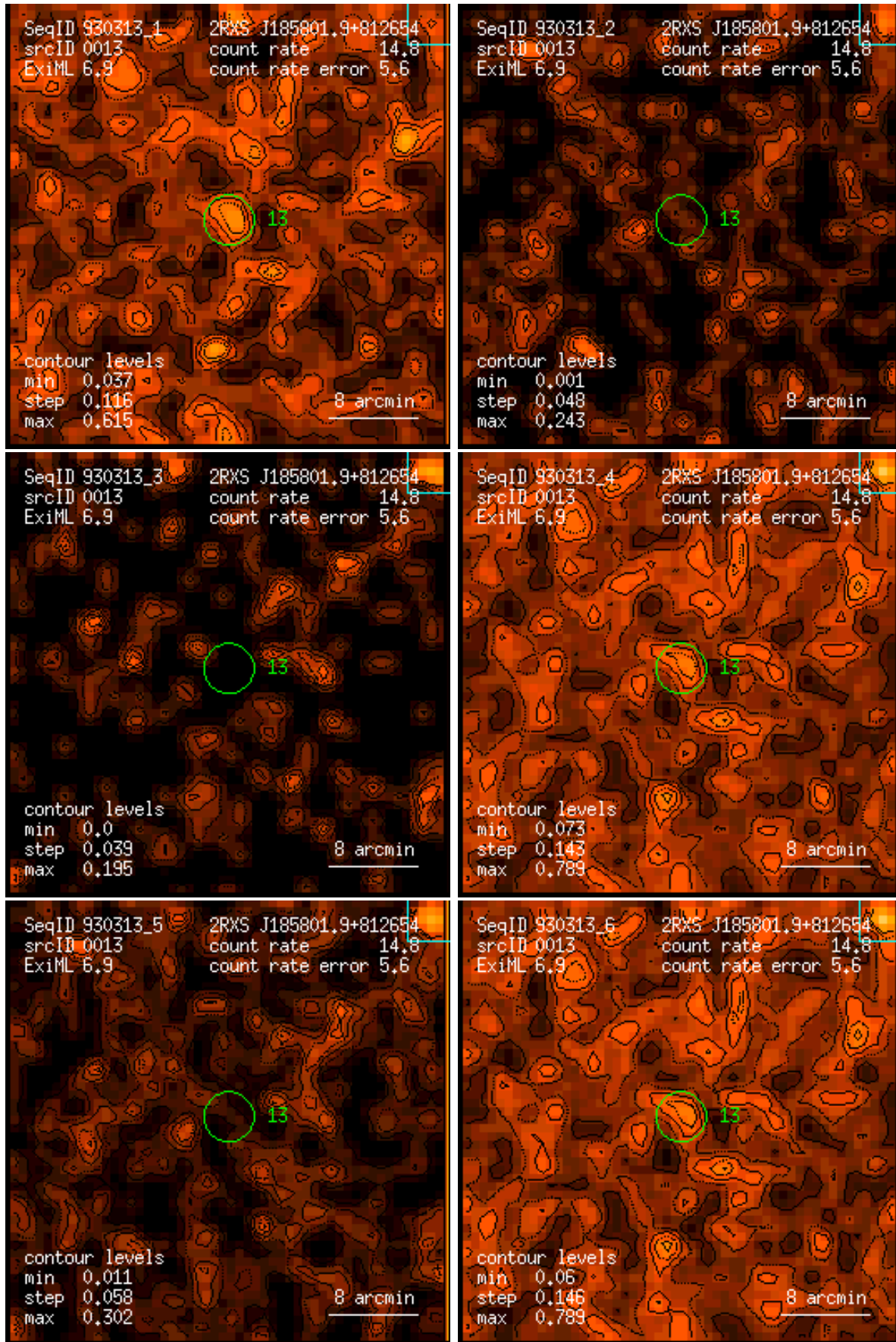
Figure 13: RASS 930313: detection 0013: band rate images, Gaussian filter: (1) PSPC channels 11 – 41, (2) 52 – 90, (3) 91 – 201, (4) 11 – 235, (5) 52 – 201, (6) 11 – 201. Broad band rates in counts/ks. Band rate contour levels in counts/ks/arcmin 2 .
