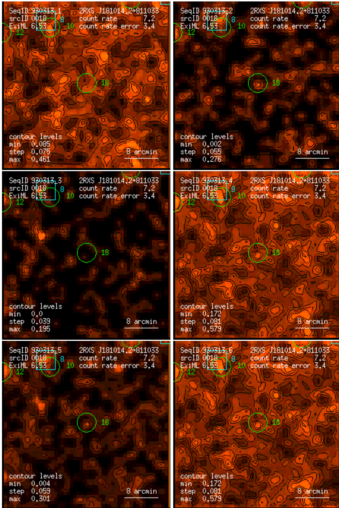
Figure 18: RASS 930313: detection 0018: band rate images, Gaussian filter: (1) PSPC channels 11 – 41, (2) 52 – 90, (3) 91 – 201, (4) 11 – 235, (5) 52 – 201, (6) 11 – 201. Broad band rates in counts/ks. Band rate contour levels in counts/ks/arcmin 2 .
